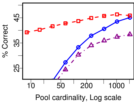
(c) 512 codewords
