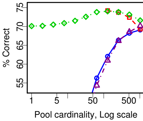
(c) 512 codewords
