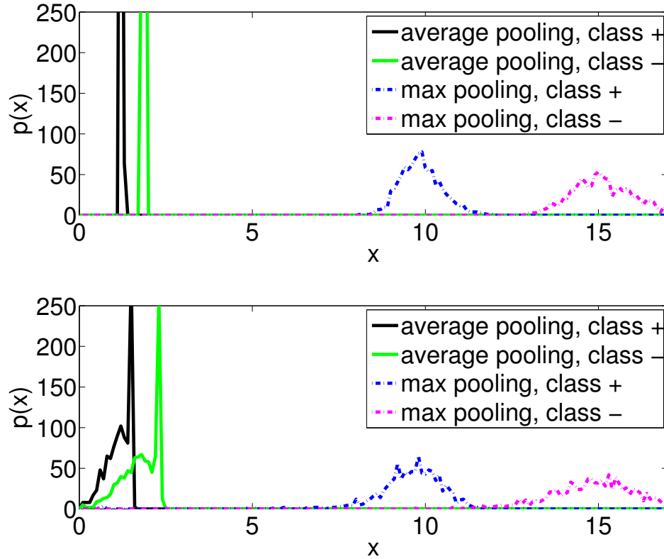
Figure 4.6: Empirical probability densities of x = \frac{1}{K} \sum_{j=1}^K h_j , simulated for two classes classes of images forming pools of cardinality N = 500 . The local features are drawn from one of three exponential distributions. When the clutter is homogeneous across images (top), the distributions are well separated for average pooling and max pooling. When the clutter level has higher variance (bottom), the max pooling distributions (dashed lines) are still well separated while the average pooling distributions (solid lines) start overlapping.
