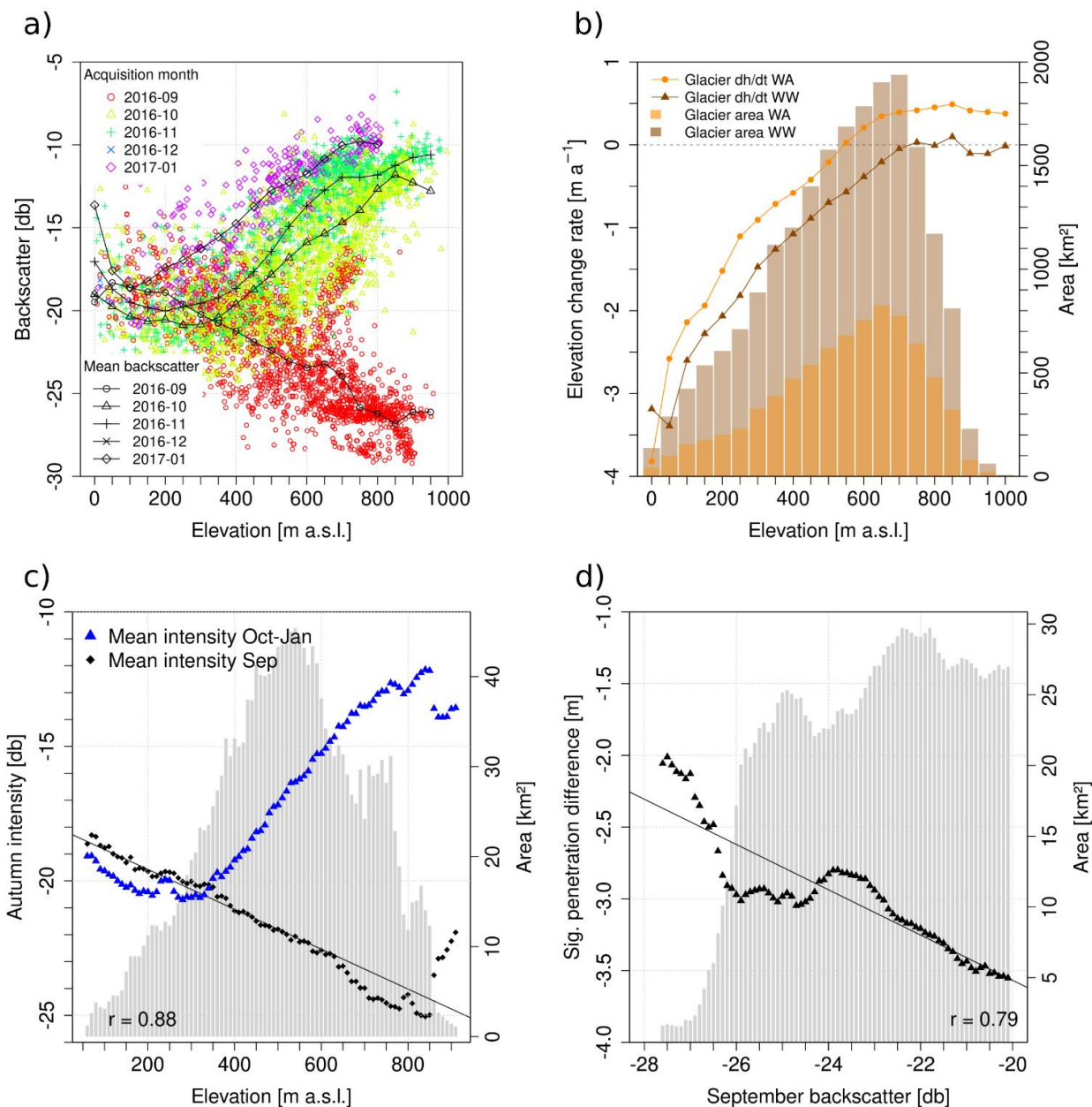
305 Figure 1 a) Backscatter intensity of different TanDEM-X DEM acquisition months versus elevation on Novaya Zemlya. Black lines indicate average backscatter aggregated within 50m elevation bins. Point icons illustrate a random subset (5000 cells) of the 2016/17 DEM mosaic of Novaya Zemlya. b) Mean elevation change rates of DEM differences between winter 2010/11 and winter 2016/17 (WW, triangles) and winter 2010/11 and September 2016 (WA, dots) of all respective glacier areas. c) Altitudinal distribution of 310 mean backscatter intensity (aggregated in 10m elevation bins) of September and winter 2016/17 SAR data on overlapping glacier areas (i.e. areas which were acquired in September and winter 2016/17). d) Differences in estimated signal penetration between September and winter 2016/17 versus mean backscatter intensity of September 2016 acquisitions on overlapping glacier areas (ag- gregated within 0.1 db backscatter intervals between -20 to -28 db). The linear correlations of mean September backscatter intensity and elevation (1c) and mean difference in signal penetration depth and September backscatter intensity (1d) are indicated as black solid lines.
