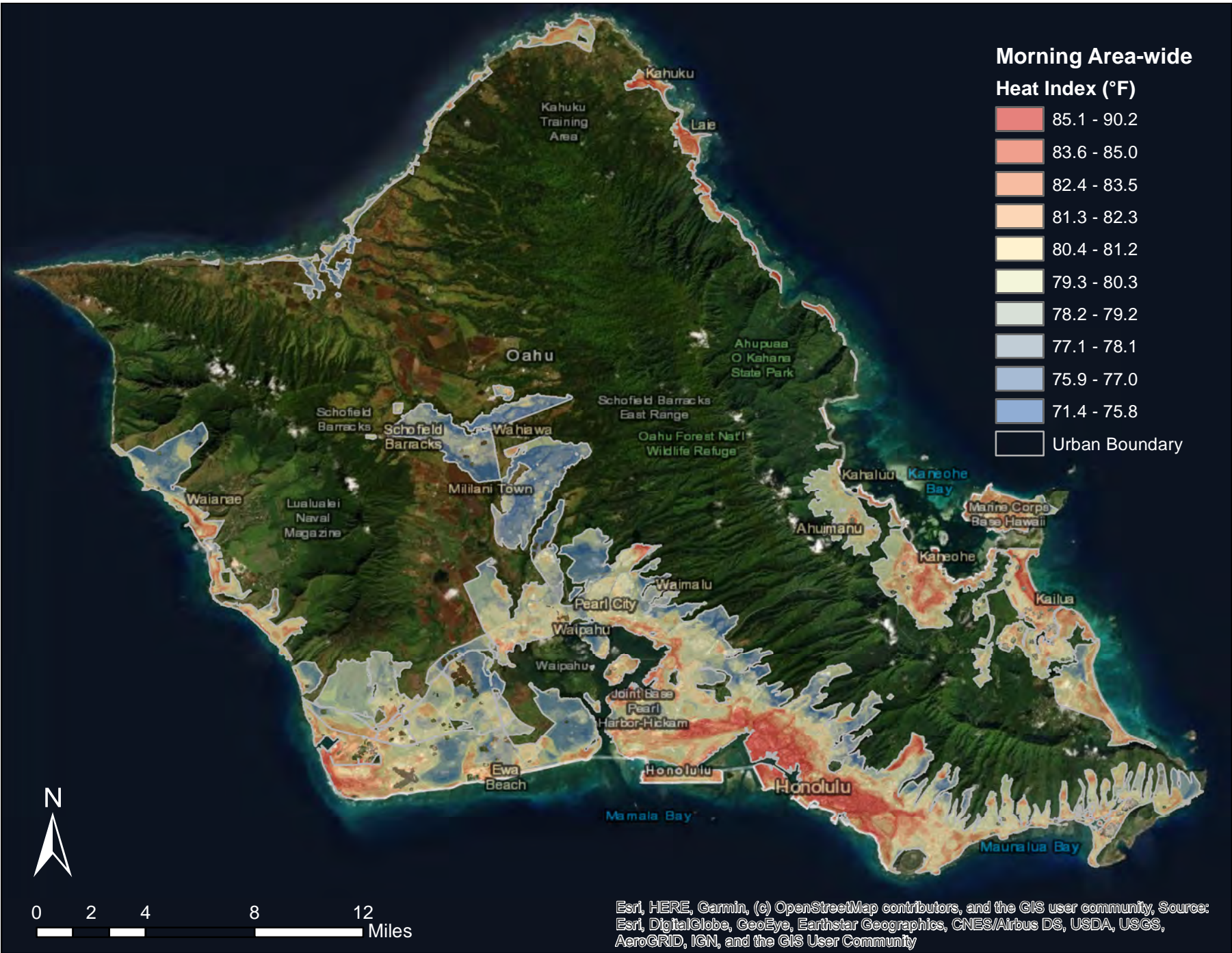
Figure 4: Honolulu 6-7AM Area-Wide Heat Index (°F)
