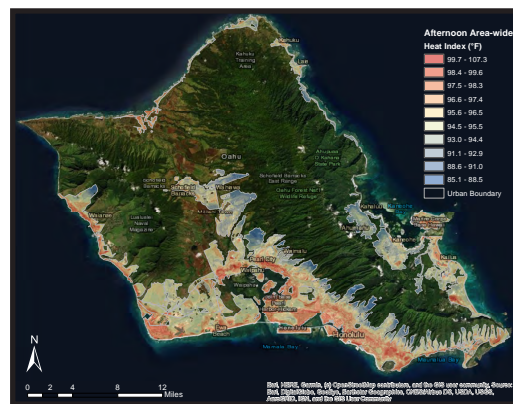
Figure 2b: Afternoon Area-wide Predictions
