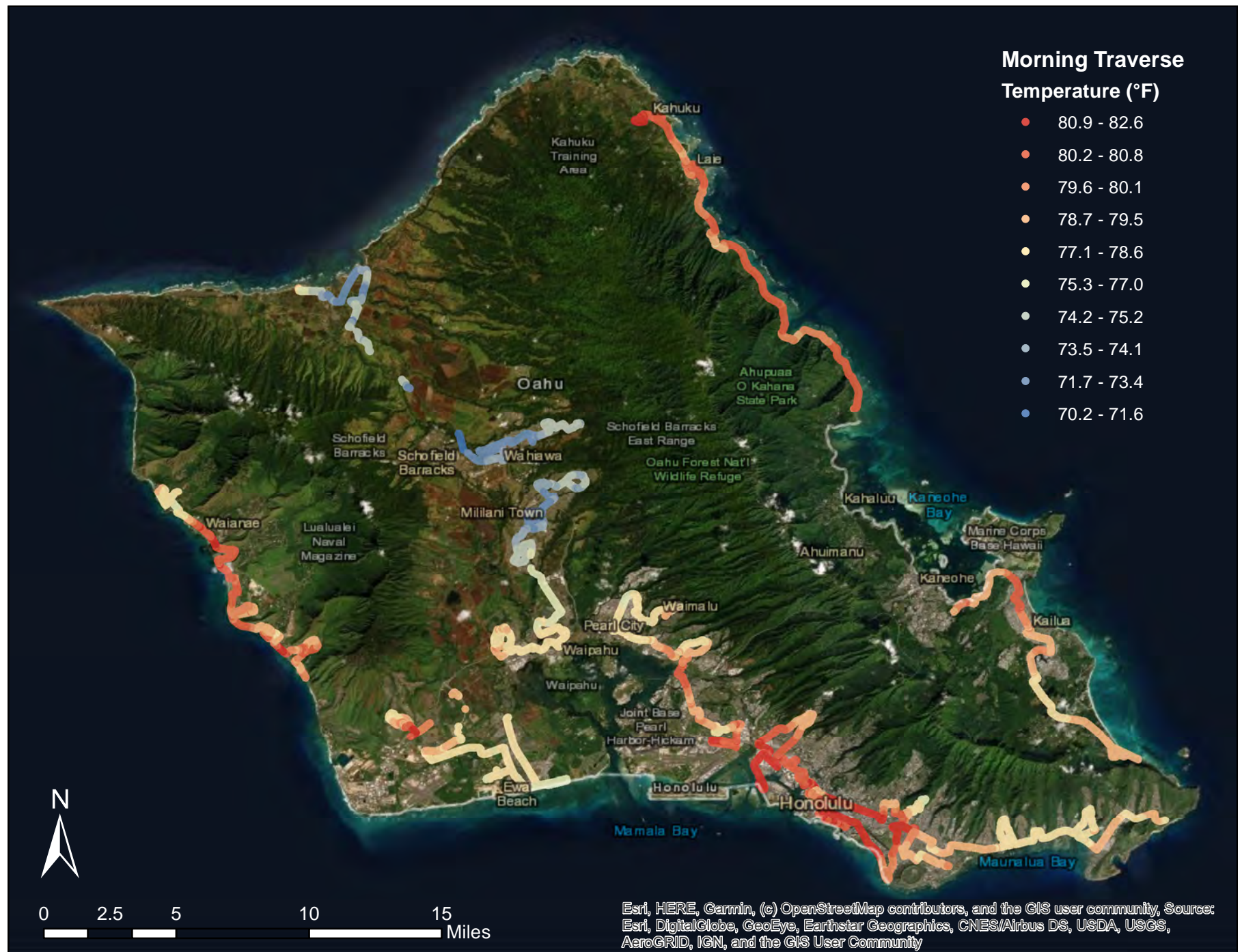
Figure 3: Honolulu 6-7AM Traverse Point Temperature (°F)
