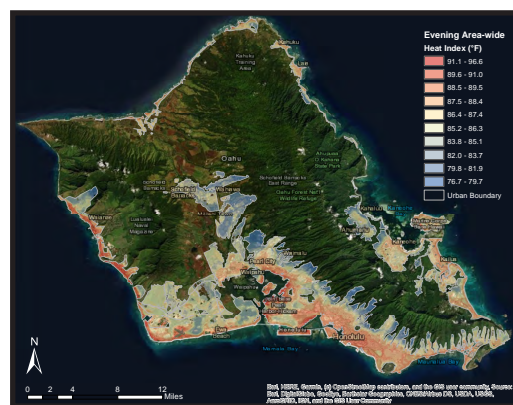
Figure 2c: Evening Area-wide Predictions
