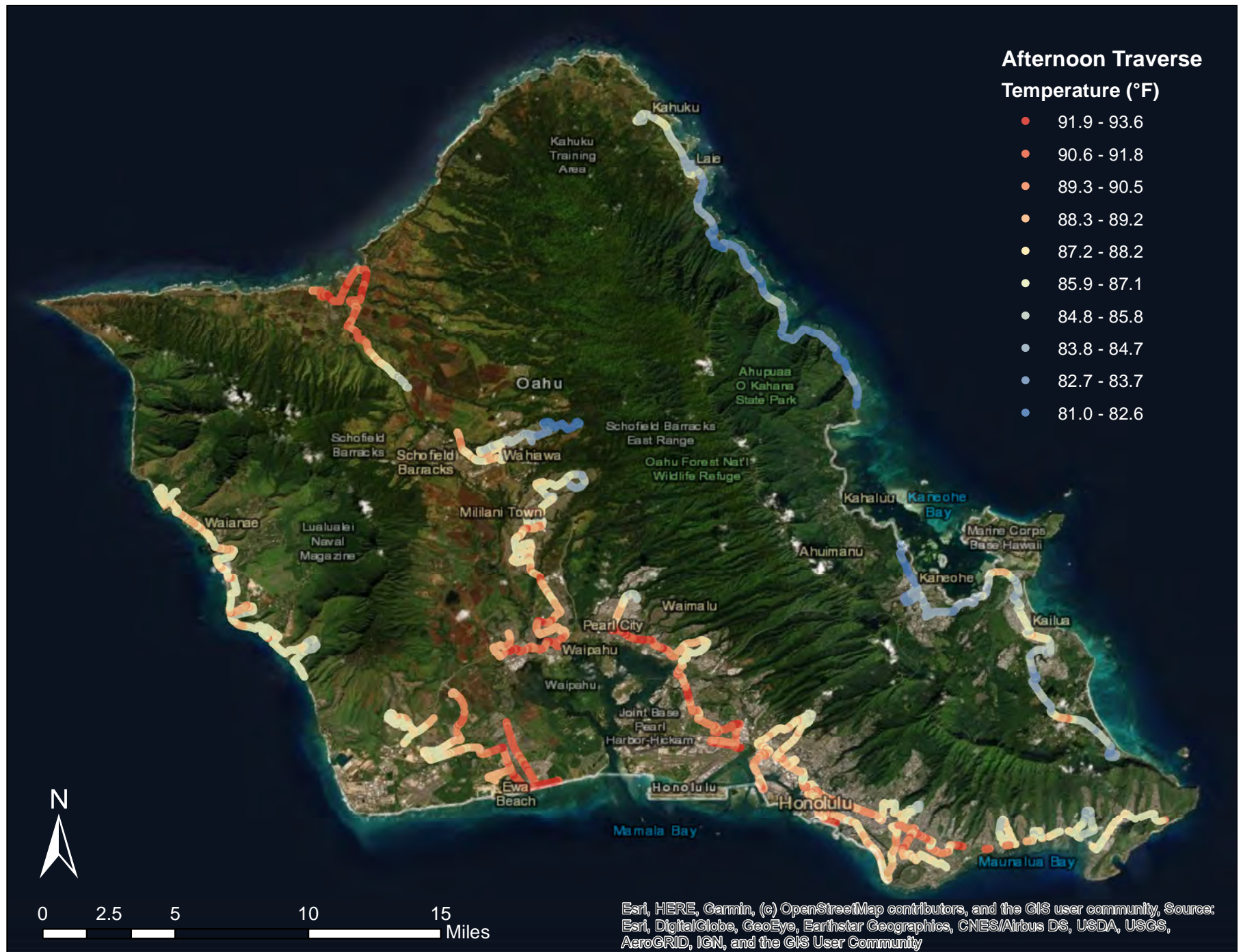
Figure 5: Honolulu 3-4PM Traverse Point Temperature (°F)
