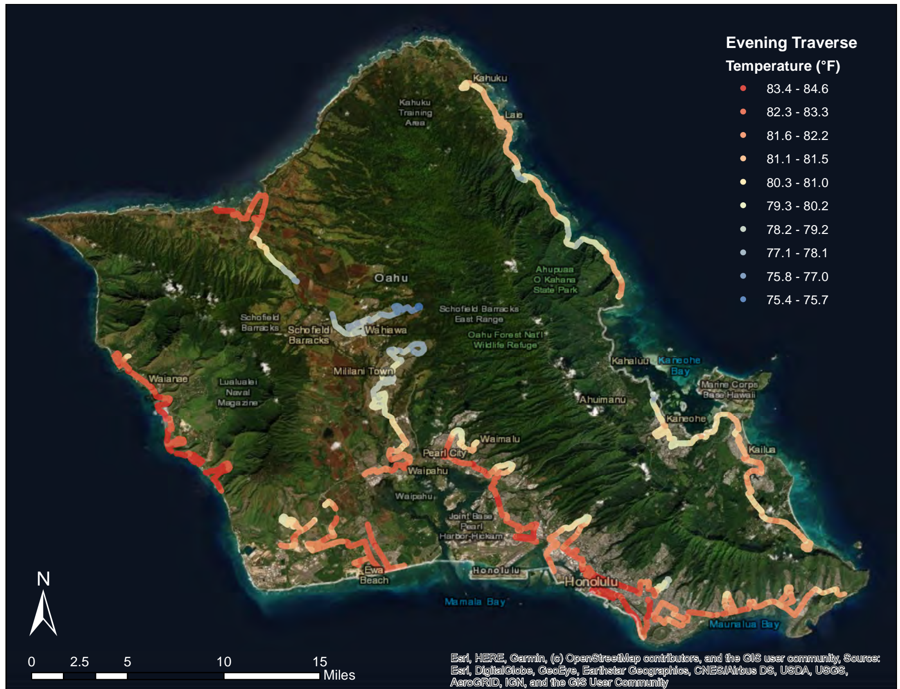
Figure 7: Honolulu 7-8PM Traverse Point Temperature (°F)
