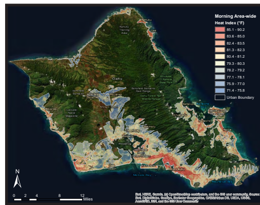
Figure 2a: Morning Area-wide Predictions
