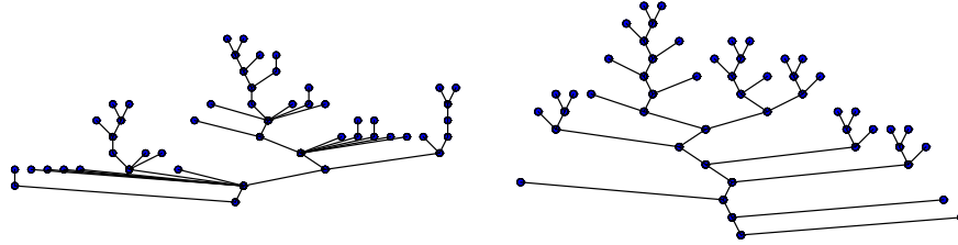
FIGURE 10. A general tree of \mathcal{G}_{51} (left) and a binary tree of \mathcal{T}_{51}^{\{0,2\}} (right) drawn uniformly at random amongst the C_{50} and C_{25} possible trees respectively, with C_n = \frac{1}{n+1} \binom{2n}{n} the n th Catalan number.
