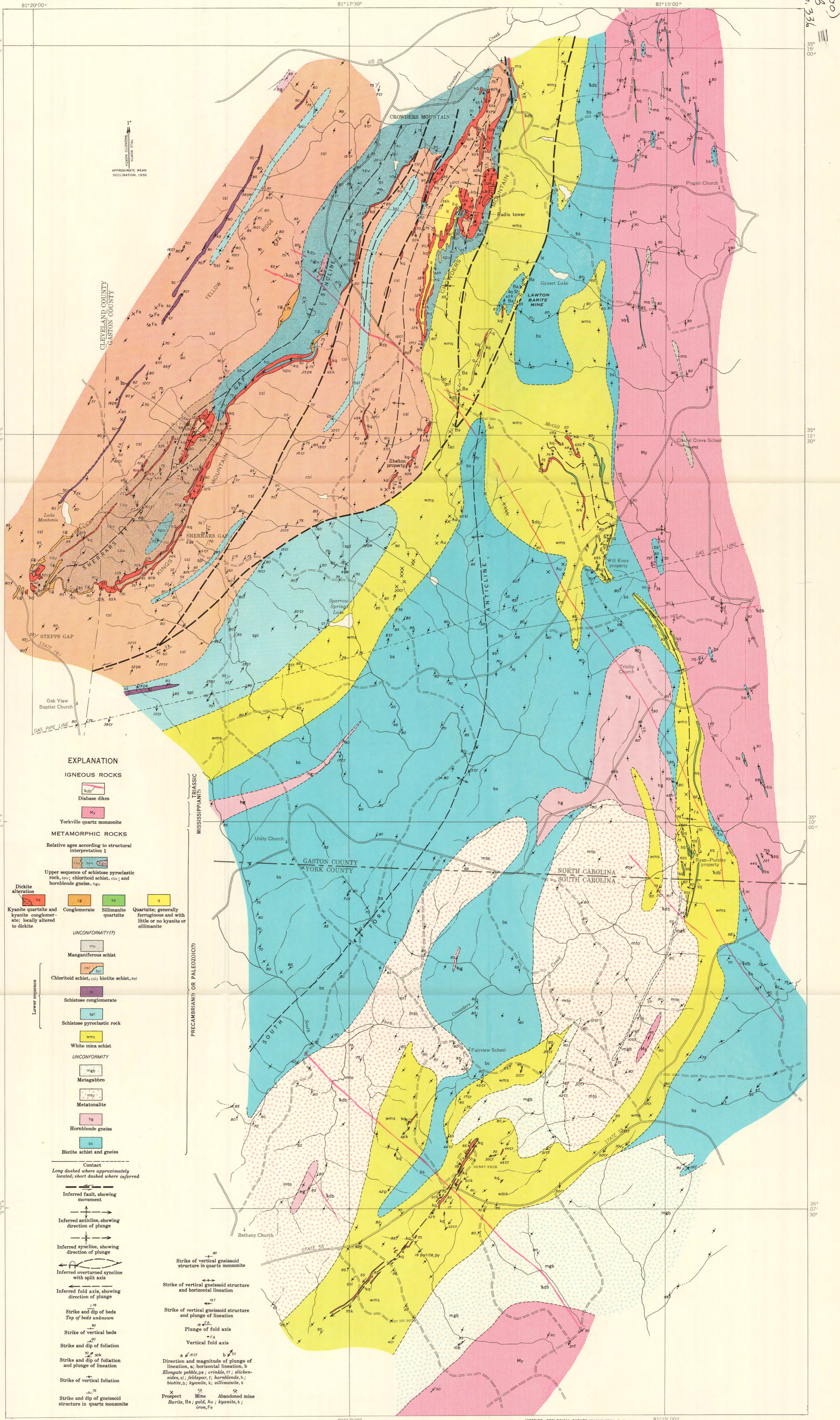
Map compiled by U. S. Geological Survey from aerial photographs. INFERIOR—GEOLOGICAL SURVEY, WASHINGTON, D. C. HR 7407. Geology mapped by D. B. Potter, 1951-52.
