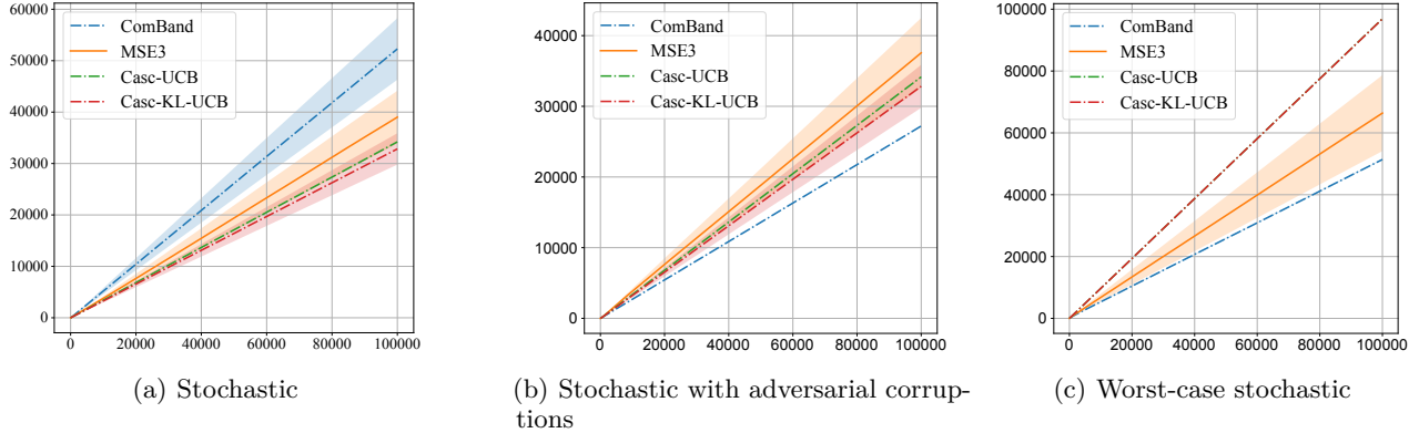
Figure 1: Cumulative reward over time in the three environment settings is described. The results also display the 95% confidence intervals over 35 runs with an Intel Xeon Gold 6312U, calculated using the standard error multiplied by the z -score of 1.96.
