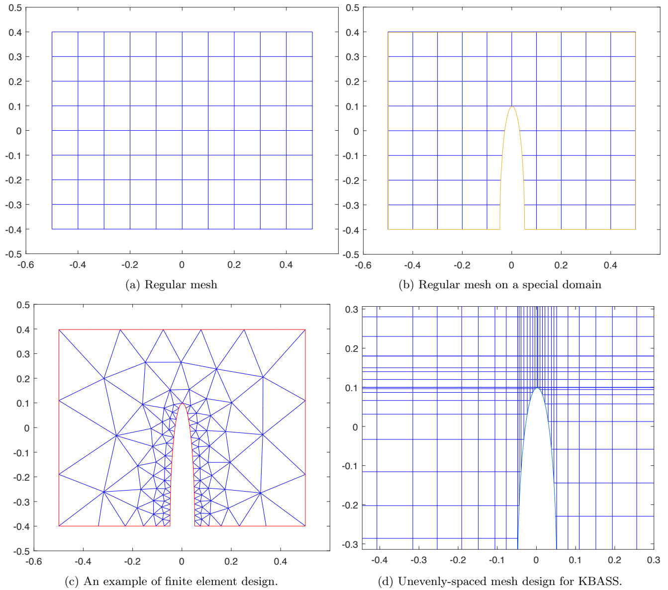
Figure 8: An example of the mesh design. By varying the density regions of the mesh (d), our method can adapt to the geometry of specific domains, as the traditional numerical methods do (c).
