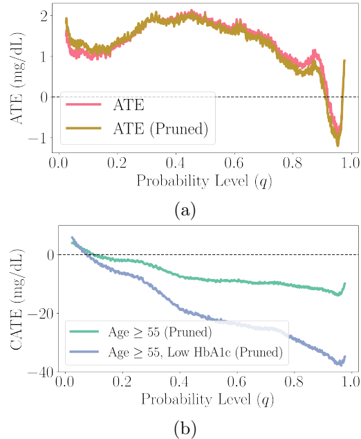
Figure 5: (a) Average treatment effect of glucose-monitoring with CGM on the distribution of glucose concentrations before pruning positivity violations (pink) and after (gold). (b) Conditional average treatment effect of glucose monitoring with CGM on the distribution of glucose concentrations for patients older than 55 years of age (green) and for those with low HbA1c levels at baseline (blue). The x-axes display the probability level and the y-axes display the difference in the related quantiles of the outcomes.
