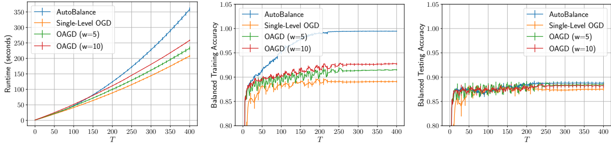
Figure 5: Performance comparison (mean±std) on parametric loss tuning for imbalanced Tadpole data over five runs. We compare our OAGD ( w = 5, 10 ) with AutoBalance and Single-Level OGD. OAGD achieves comparable balanced testing accuracy to AutoBalance but with a reduced runtime.
