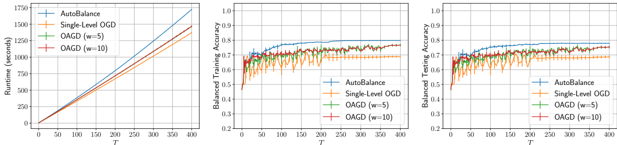
Figure 6: Performance comparison (mean±std) on parametric loss tuning for imbalanced Adult data over five runs. We compare our OAGD ( w = 5, 10 ) with AutoBalance and Single-Level OGD. OAGD achieves comparable balanced testing accuracy to AutoBalance but with a reduced runtime.
