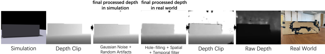
Figure 5: We bridge the visual gap between simulation and real world by applying pre-processing techniques. We use depth clipping, Gaussian noise and random artifacts in simulation, and depth clipping and hole-filling, spatial and temporal filters in the real world.
