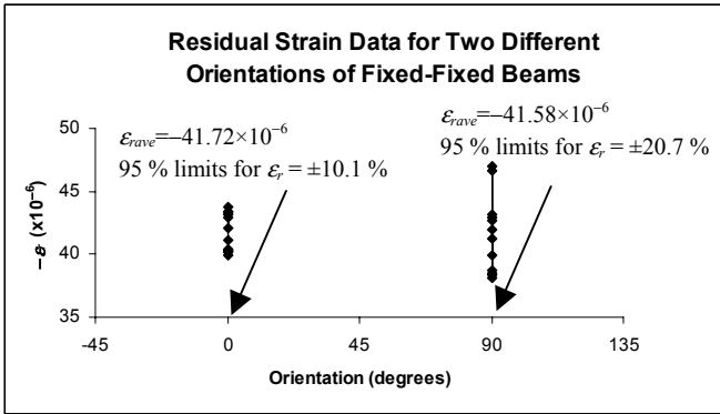
Figure 12. A plot of -\epsilon_r versus orientation.
