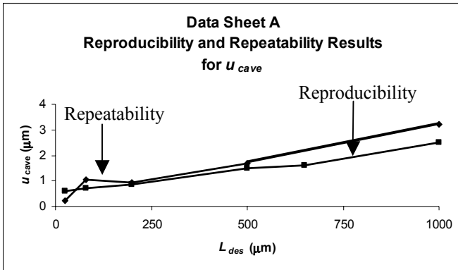
Figure 10. Comparing reproducibility and repeatability results for u_{cave} in Data Sheet A.
