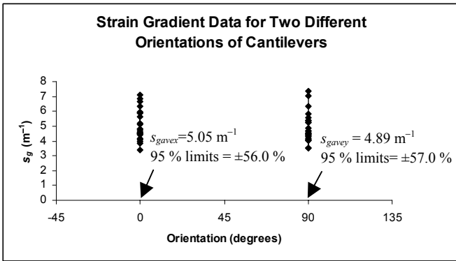
Figure 14. A plot of s_g versus orientation.
