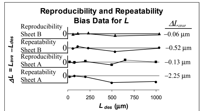
Figure 9. Reproducibility and repeatability bias data for L .
