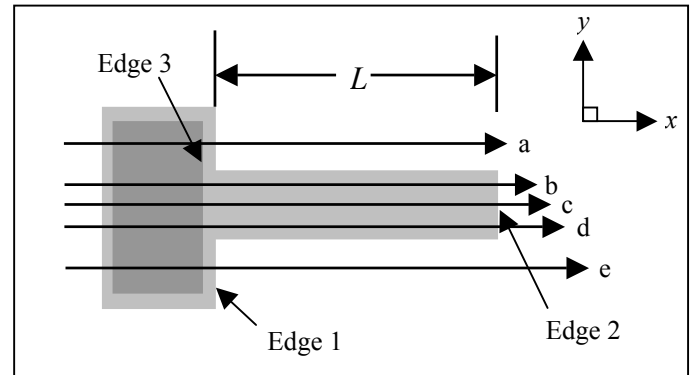
Figure 6. Top view of a cantilever test structure.
