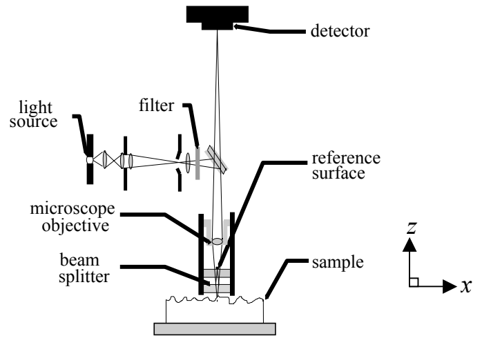
Figure 4. Schematic of an optical interferometer.
