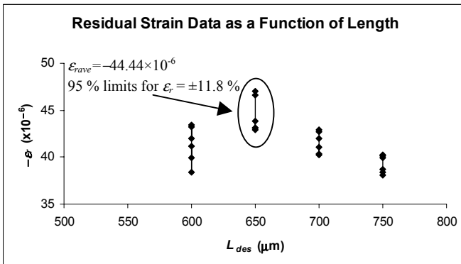
Figure 13. A plot of -\epsilon_r versus length.
