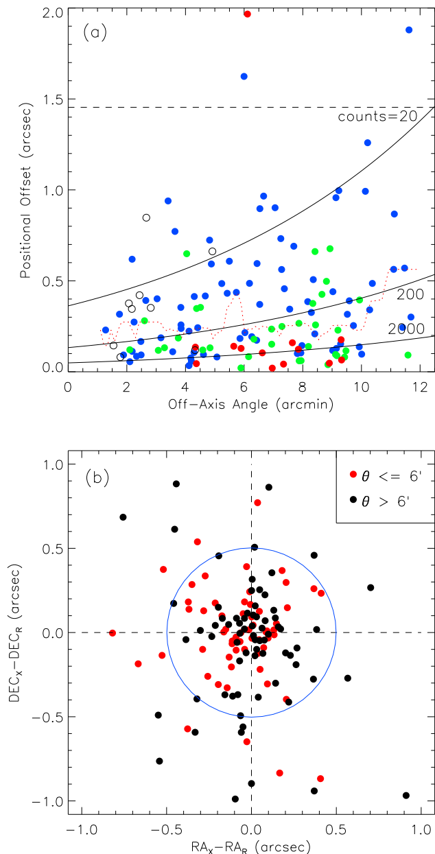
FIG. 6.— (a) Positional offset vs. off-axis angle for the 135 main-catalog sources that have counterparts in the 5\sigma VLA 1.4 GHz radio catalog using a matching radius of 2'' (see § 4.2 for descriptions of the three sources with > 1.5'' positional offsets). Red filled, green filled, blue filled, and black open circles represent X-ray sources with \geq 2000 , \geq 200 , \geq 20 , and < 20 counts in the energy band where the source position was determined, respectively. The red dotted curve shows the running median of positional offset in bins of 2' . The horizontal dashed line indicates the median offset ( 1.45'' ) of the expected false matches. We used these data to derive the \approx 68\% confidence-level X-ray source positional uncertainties, i.e., eq. (2). Three solid curves indicate the \approx 68\% confidence-level positional uncertainties for sources with 20, 200 and 2000 counts. (b) Positional residuals between the X-ray and radio positions for the 132 main-catalog sources that have radio counterparts within a radius of 1.5'' [see Panel (a)]. Red and black filled circles indicate sources with an off-axis angle of \leq 6' and > 6' , respectively. A large blue circle with a radius of 0.5'' is drawn at the center as a guide to the eyes. [see the electronic edition of the Supplement for a color version of this figure.]
