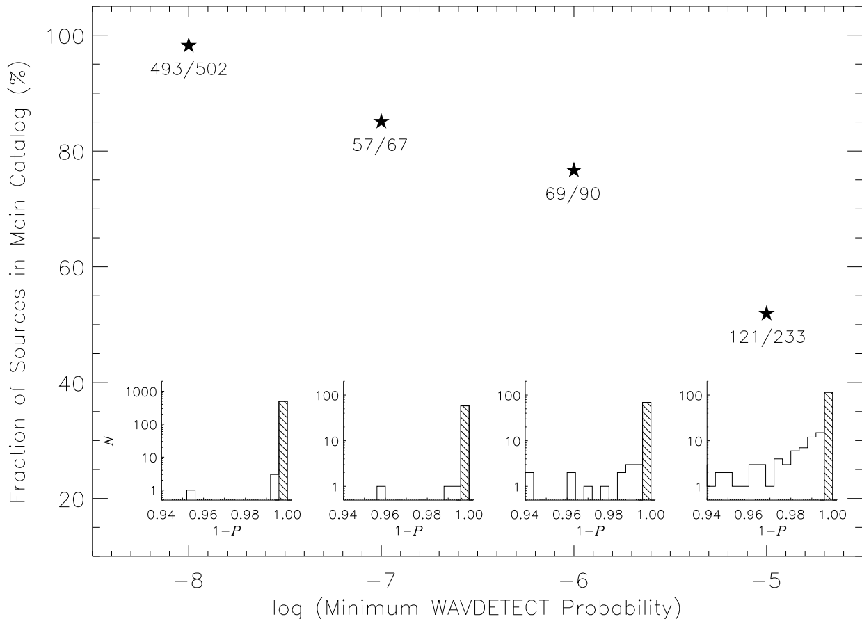
FIG. 5.— The fraction of sources in the candidate-list catalog with an AE binomial no-source probability P < 0.004 , which were included in the main catalog, as a function of minimum WAVDETECT probability 38 (shown as five-pointed stars). The number of sources with P < 0.004 versus the number of candidate-list catalog sources detected at each minimum WAVDETECT probability are annotated in the figure (note that, in this figure, 502+67+90+233=892 and 493+57+69+121=740 ). The fraction of candidate-list catalog sources included in the main catalog falls from 98.2% to 51.9% between minimum WAVDETECT probabilities of 10^{-8} and 10^{-5} . Shown in the insets are the histograms of 1-P for the candidate-list catalog sources at each minimum WAVDETECT probability, with shaded areas highlighting those included in the main catalog (i.e., having 1-P > 0.996 ).
