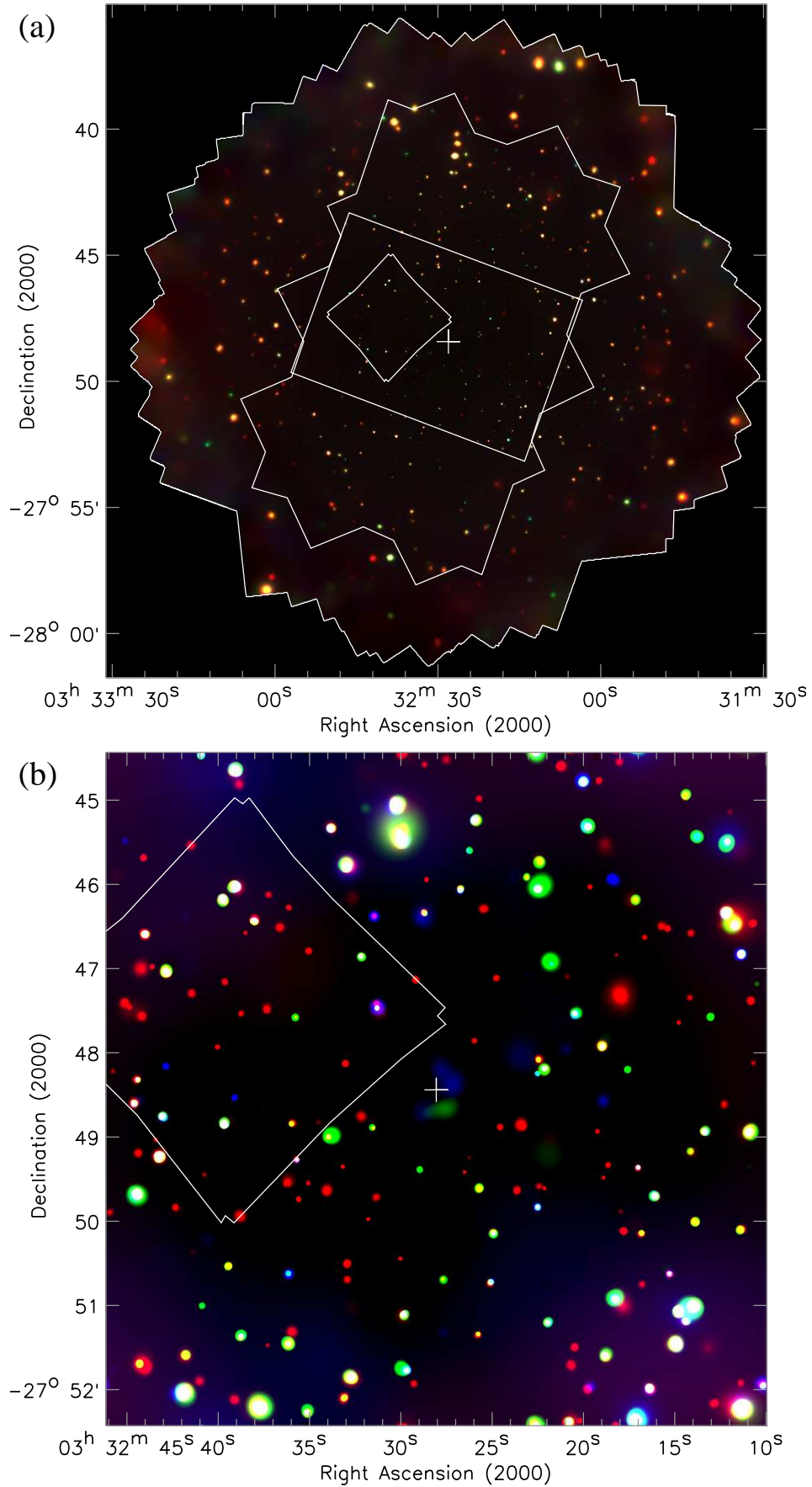
FIG. 4.— (a) Chandra “false-color” image of the 4 Ms CDF-S, which is a color composite of the exposure-corrected and adaptively smoothed images in the 0.5–2.0 keV (red), 2–4 keV (green), and 4–8 keV (blue) bands. (b) An expanded view of the Chandra “false-color” image of the central 8' \times 8' region (note that a slightly different contrast ratio from that for the full image is used here in order to render the faint sources more clearly). The apparent smaller size and lower brightness of sources near the field center is due to the smaller size of the on-axis PSF. The regions and the plus sign are the same as those in Fig. 1.
