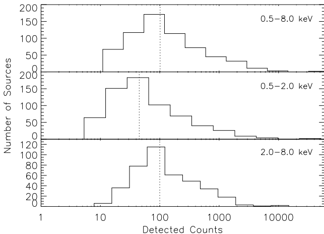
FIG. 9.— Histograms of detected source counts for the main-catalog sources in the full (top), soft (middle), and hard (bottom) bands. Sources with upper limits have not been included in the plots. The vertical dotted lines indicate median numbers of counts in each band (see Table 4).
