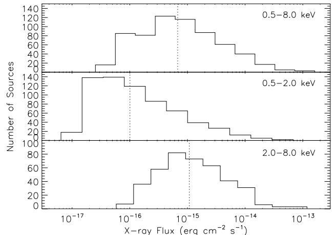
FIG. 10.— Histograms of X-ray fluxes for the main-catalog sources in the full (top), soft (middle), and hard (bottom) bands. Sources with upper limits have not been included in the plots. The vertical dotted lines indicate the median fluxes of 6.8 \times 10^{-16} , 1.0 \times 10^{-16} and 1.1 \times 10^{-15} \text{erg cm}^{-2} \text{s}^{-1} for the full, soft, and hard bands, respectively.
