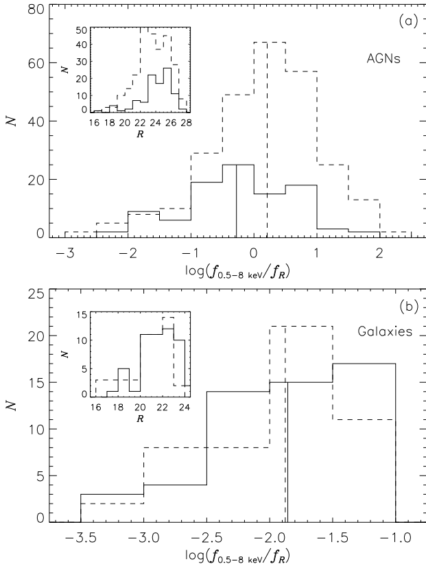
FIG. 19.— Distributions of X-ray-to-optical flux ratio for (a) new AGNs (solid histogram) and old AGNs (dashed histogram) and (b) new galaxies (solid histogram) and old galaxies (dashed histogram) with median flux ratios indicated by vertical lines. Shown in the insets are the distributions of R -band magnitude for new AGNs/galaxies (solid histograms) and old AGNs/galaxies (dashed histograms). Only sources with both full-band and R -band detections are shown.
