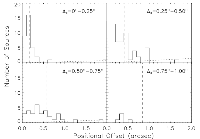
FIG. 7.— Histograms showing the distributions of positional offset for the 135 main-catalog sources that have counterparts in the 5\sigma VLA 1.4 GHz radio catalog using a matching radius of 2'' . These 135 sources were divided into four bins according to their positional uncertainties estimated using eq. (2): 0''-0.25'' , 0.25''-0.50'' , 0.50''-0.75'' , and 0.75''-1'' . The vertical dashed line in each panel indicates the median X-ray positional uncertainty in each bin. The dotted line shows the total expected number of random radio sources as a function of the positional offset. \lesssim 35\% of the radio counterparts lie beyond the median X-ray positional uncertainty in each bin.
