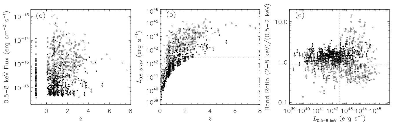
FIG. 14.— Plots of (a) observed-frame full-band flux vs. redshift, (b) absorption-corrected, rest-frame 0.5–8 keV luminosity vs. redshift, and (c) band ratio vs. absorption-corrected, rest-frame 0.5–8 keV luminosity, for the main-catalog sources. Gray open circles indicate the main-catalog sources that were previously detected in the L08 main catalog; black filled circles indicate the new main-catalog sources that were not previously detected in the L08 main catalog. Arrows indicate limits. Several sources shown in Panels (a) and (b) have photometric redshifts greater than \approx 4.5 ; these photometric redshifts are probably not very reliable due to poor photometric coverage (see § 3.3 of L10 for more discussion). In Panel (b), sources without redshift estimates have not been included in the plot; in Panel (c), sources without redshift estimates and sources with only full-band detections have not been included in the plot. The dotted lines in Panels (b, c) and the dashed-dot line in Panel (c) indicate the threshold values of two AGN-identification criteria (i.e., L_{0.5-8 \text{ keV}} \geq 3 \times 10^{42} \text{ erg s}^{-1} and \Gamma \leq 1.0 ; see the description of Column 78 for details).
