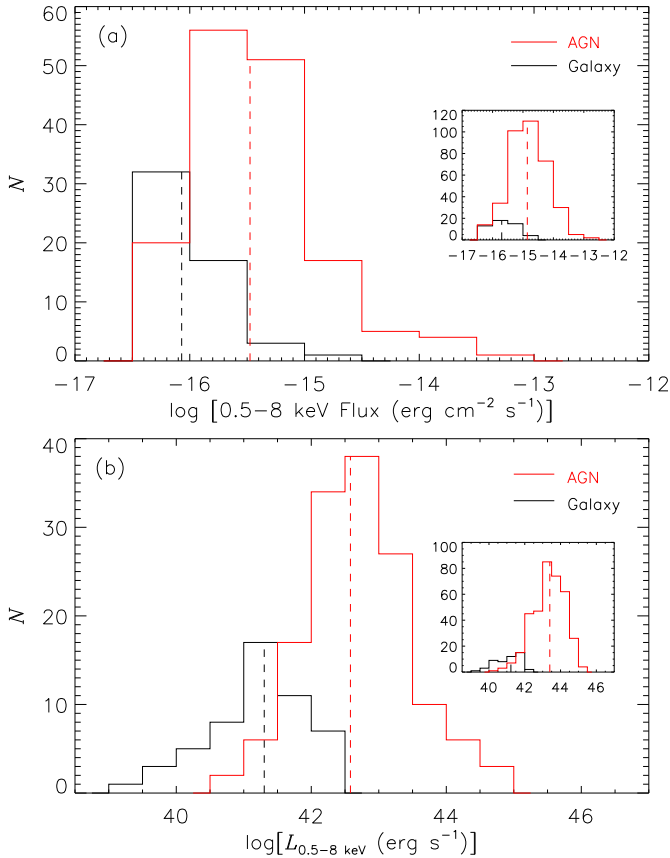
FIG. 15.— Distributions of (a) observed-frame full-band flux and (b) absorption-corrected, rest-frame 0.5–8 keV luminosity for the new main-catalog sources. The red and black histograms indicate AGNs and galaxies, respectively. The vertical red and black dashed lines indicate the median values for AGNs and galaxies, respectively. Sources with upper limits on full-band fluxes have not been included in the plotting for panel (a); sources without estimates of X-ray luminosities (due to no available redshift) or with upper limits on X-ray luminosities have not been included in the plotting for panel (b). The insets show results for the old main-catalog sources. [see the electronic edition of the Supplement for a color version of this figure.]
