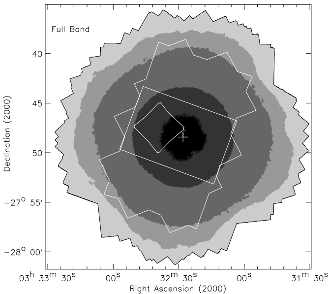
FIG. 22.— Full-band sensitivity map for the main catalog, created following § 7.2. The gray-scale levels, from black to light gray, represent areas with flux limits of < 4.0 \times 10^{-17} , 4.0 \times 10^{-17} to 10^{-16} , 10^{-16} to 3.3 \times 10^{-16} , 3.3 \times 10^{-16} to 10^{-15} , and > 10^{-15} \text{erg cm}^{-2} \text{s}^{-1} , respectively. The regions and the plus sign are the same as those in Fig. 1.
