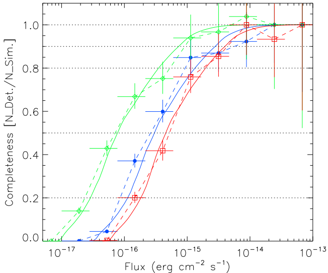
FIG. 21.— Completeness as a function of flux under the main-catalog P < 0.004 criterion for the simulations in the full (blue filled circles), soft (green open diamonds), and hard (red open squares) bands, overlaid with the corresponding sky coverage curves (solid curves) calculated in § 7.3 and normalized to the maximum sky coverage (see the solid curves in Fig. 23). The dashed lines connect the corresponding cross points. The horizontal dotted lines indicate five completeness levels. [see the electronic edition of the Supplement for a color version of this figure.]
