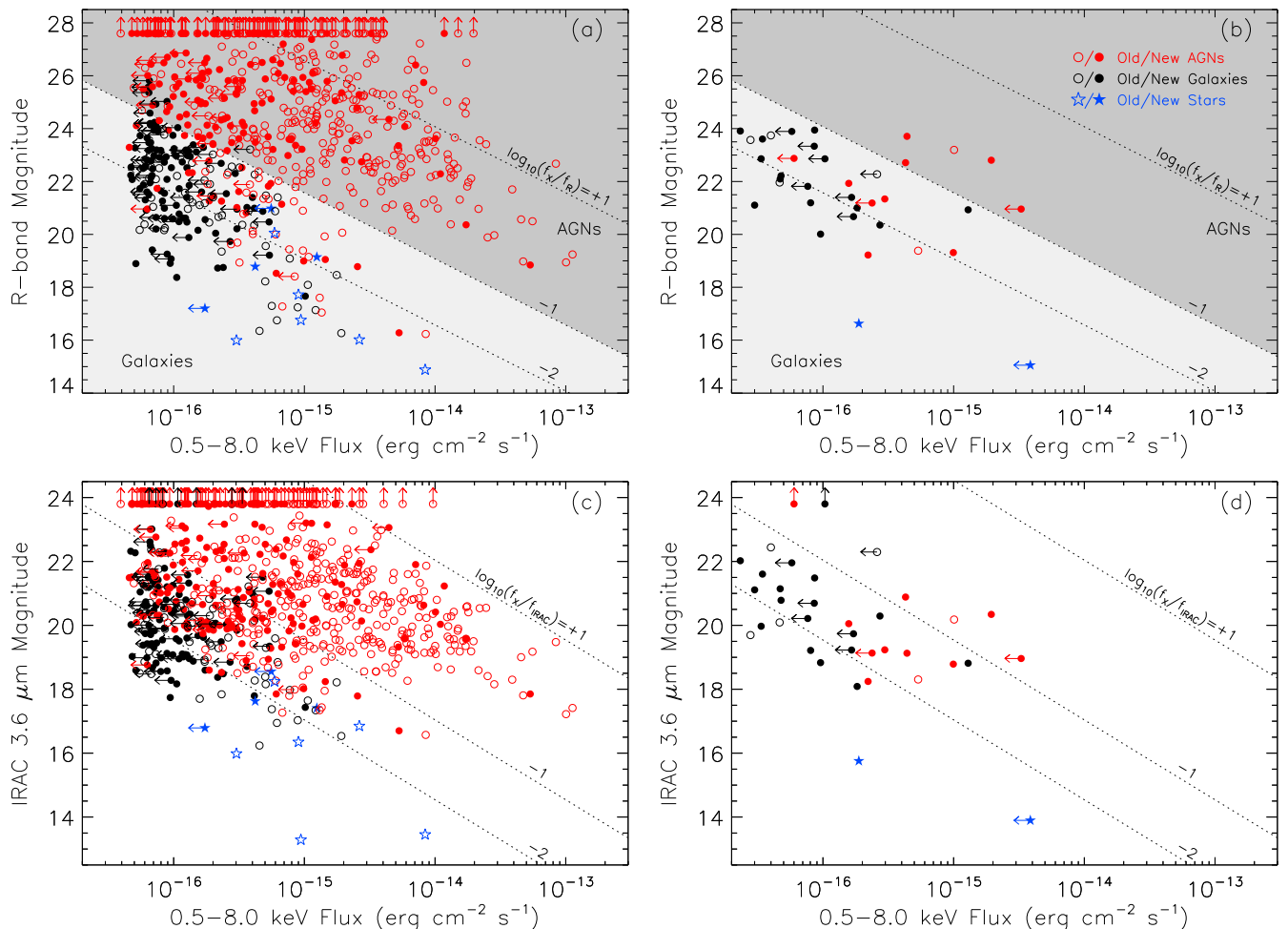
FIG. 18.— (Top) WFI R -band magnitude vs. full-band flux for sources in (a) the main catalog and (b) the supplementary optically bright catalog [note that the legend in Panel (b) applies for all the panels in this figure]. Sources that are considered AGNs, galaxies, and stars are colored red, black, and blue, respectively. Open circles indicate AGNs/galaxies that were previously detected in (a) the L08 main catalog or (b) the L08 main or supplementary optically bright catalog; open stars in (a) indicate stars that were previously detected in the L08 main catalog; filled circles and stars indicate new AGNs/galaxies and stars, respectively. Arrows indicate limits. Diagonal lines indicate constant flux ratios between the WFI R -band and the full band, with the shaded areas showing the approximate flux ratios for AGNs (dark gray) and galaxies (light gray). (Bottom) IRAC 3.6 \mu\text{m} magnitude vs. full-band flux for sources in (c) the main catalog and (d) the supplementary optically bright catalog. All the symbols are the same as those in Panels (a) and (b). The diagonal lines indicate constant flux ratios between the IRAC 3.6 \mu\text{m} band and the full band. Note that several galaxies that have R -band detections were not detected in the IRAC 3.6 \mu\text{m} band, probably due to source blending in the IRAC 3.6 \mu\text{m} band and/or these galaxies being very blue systems. [see the electronic edition of the Supplement for a color version of this figure.]
