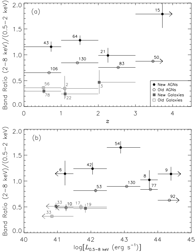
FIG. 17.— Average (i.e., stacked) band ratio in bins of (a) redshift ( 0 < z < 1 , 1 \leq z < 2 , 2 \leq z < 3 , and z \geq 3 ) and (b) X-ray luminosity [ \log(L_X) < 41.5 , 41.5 \leq \log(L_X) < 42.5 , 42.5 \leq \log(L_X) < 43.5 , 43.5 \leq \log(L_X) < 44.0 , and \log(L_X) \geq 44.0 ] for new AGNs (filled circles), old AGNs (open circles), new galaxies (filled squares), and old galaxies (open squares). The median redshift or X-ray luminosity in each bin is used for plotting. The number of stacked sources in each redshift or luminosity bin is annotated.
