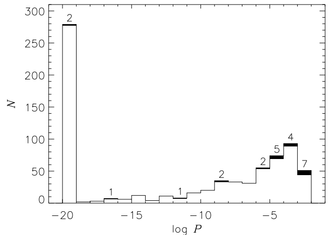
FIG. 11.— Histogram of the AE-computed binomial no-source probability, P , for the main-catalog sources. For the purpose of illustration, we set the values of P < 10^{-20} to P = 10^{-20} in this plot. The shaded areas indicate sources that have no multiwavelength counterparts, with the numbers of these unidentified sources listed above the corresponding shaded areas.
