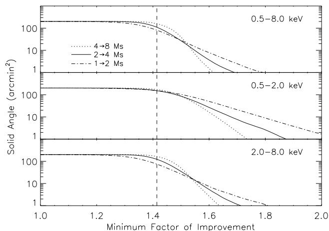
FIG. 24.— Survey solid angle within the central \theta = 8' area as a function of minimum factor of improvement in sensitivity in the three standard bands under the source-detection criterion P < 0.004 . The improvement curves for the cases of 1 to 2 Ms, 2 to 4 Ms, and 4 to 8 Ms are shown as dash-dot, solid, and dotted curves, respectively; the curves for the first two cases are calculated using real data, while the curves for the third case are simulated (see § 7.3). The vertical dashed lines indicate a factor of \sqrt{2} improvement in sensitivity that is expected for each doubling of exposure time in a background-limited case under the assumption, here inapplicable, of Gaussian statistics.
