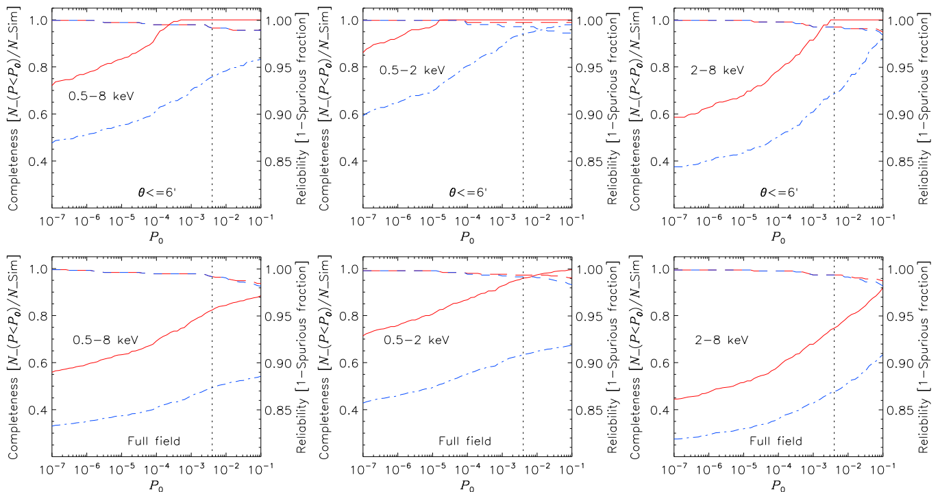
FIG. 20.— (Top) Case of \theta < 6' : completeness (solid and dashed-dot curves; left y-axis) and reliability (long dashed and short dashed curves; right y-axis) as a function of P_0 , the AE-computed binomial no-source probability threshold chosen for detection, for the simulations in the full, soft, and hard bands, for sources with at least 15 counts (red solid and long dashed curves) and at least 8 counts (blue dashed-dot and short dashed curves), respectively. Note that the short dashed curves overlap almost exactly along the long dashed curves in some cases (e.g., top-left and top-right panels). The vertical dotted lines indicate the chosen main-catalog source-detection threshold of P_0 = 0.004 . (Bottom) Same as top panels, but for the entire CDF-S field. [see the electronic edition of the Supplement for a color version of this figure.]
