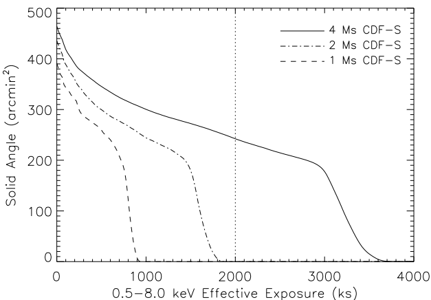
FIG. 3.— Plot of survey solid angle as a function of minimum full-band effective exposure for the 4 Ms CDF-S (solid curve). The maximum exposure is 3.811 Ms. The vertical dotted line indicates an effective exposure of 2 Ms. Approximately 242.3 arcmin 2 ( \approx 52\% ) of the CDF-S survey area has > 2 Ms effective exposure. For comparison, the 1 Ms CDF-S result (dashed curve) and the 2 Ms CDF-S result (dash-dot curve), both of which are obtained using the procedures in this paper, are also shown in the plot.
