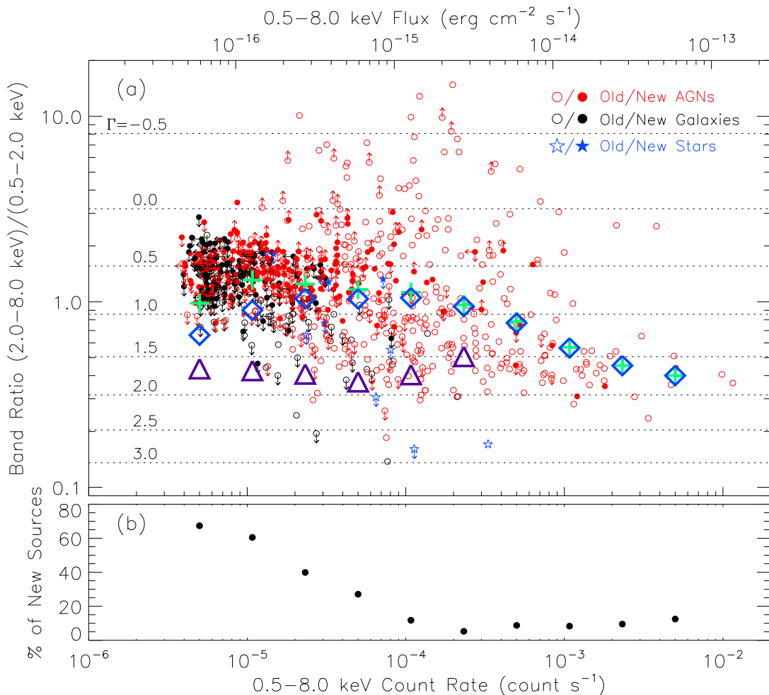
FIG. 16.— (a) Band ratio vs. full-band count rate for the main-catalog sources (for reference, the top x -axis shows representative full-band fluxes, which are derived from full-band count rates assuming a \Gamma = 1.4 power law). Sources that are considered AGNs, galaxies, and stars are colored red, black, and blue, respectively. Open circles and stars indicate AGNs/galaxies and stars that were previously detected in the L08 main catalog; filled circles and stars indicate new AGNs/galaxies and stars, respectively. Arrows indicate upper or lower limits, which mostly lie in the area of low count rates. Sources detected only in the full band cannot be plotted. Large crosses, triangles, and diamonds show average band ratios as a function of full-band count rate derived in bins of \Delta\log(\text{Count Rate}) = 0.6 from stacking analyses, for all AGNs, all galaxies, and all sources (including both AGNs and galaxies), respectively. Horizontal dotted lines show the band ratios corresponding to given effective photon indexes. (b) Fraction of new sources as a function of full-band count rate for the main-catalog sources. The fractions are calculated in bins of \Delta\log(\text{Count Rate}) = 0.6 . [see the electronic edition of the Supplement for a color version of this figure.]
