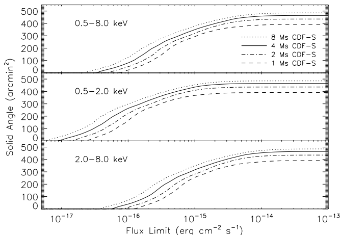
FIG. 23.— Survey solid angle as a function of flux limit in the three standard bands for the main catalog (shown as solid curves), determined following § 7.2. For comparison, the curves for the 1 Ms CDF-S (shown as dashed curves), the 2 Ms CDF-S (shown as dash-dot curves), and the simulated 8 Ms CDF-S (shown as dotted curves) are also plotted; these curves are calculated/simulated consistently (see § 7.3).
