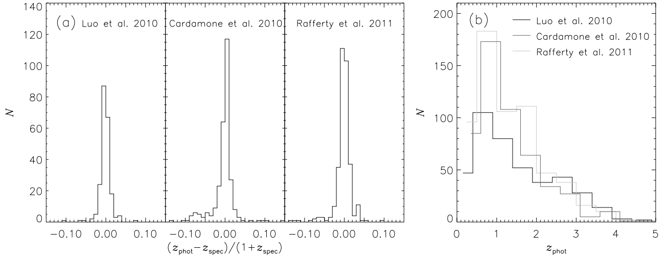
FIG. 8.— (a) Histogram of (z_{\text{phot}} - z_{\text{spec}})/(1 + z_{\text{spec}}) for L10 (218 sources), Cardamone et al. (2010; 314 sources), and Rafferty et al. (2011; 339 sources). (b) Histogram of z_{\text{phot}} for L10 (black histogram; 417 sources), Cardamone et al. (2010; dark-gray histogram; 508 sources), and Rafferty et al. (2011; light-gray histogram; 611 sources). The histograms have been slightly shifted for clarity.
