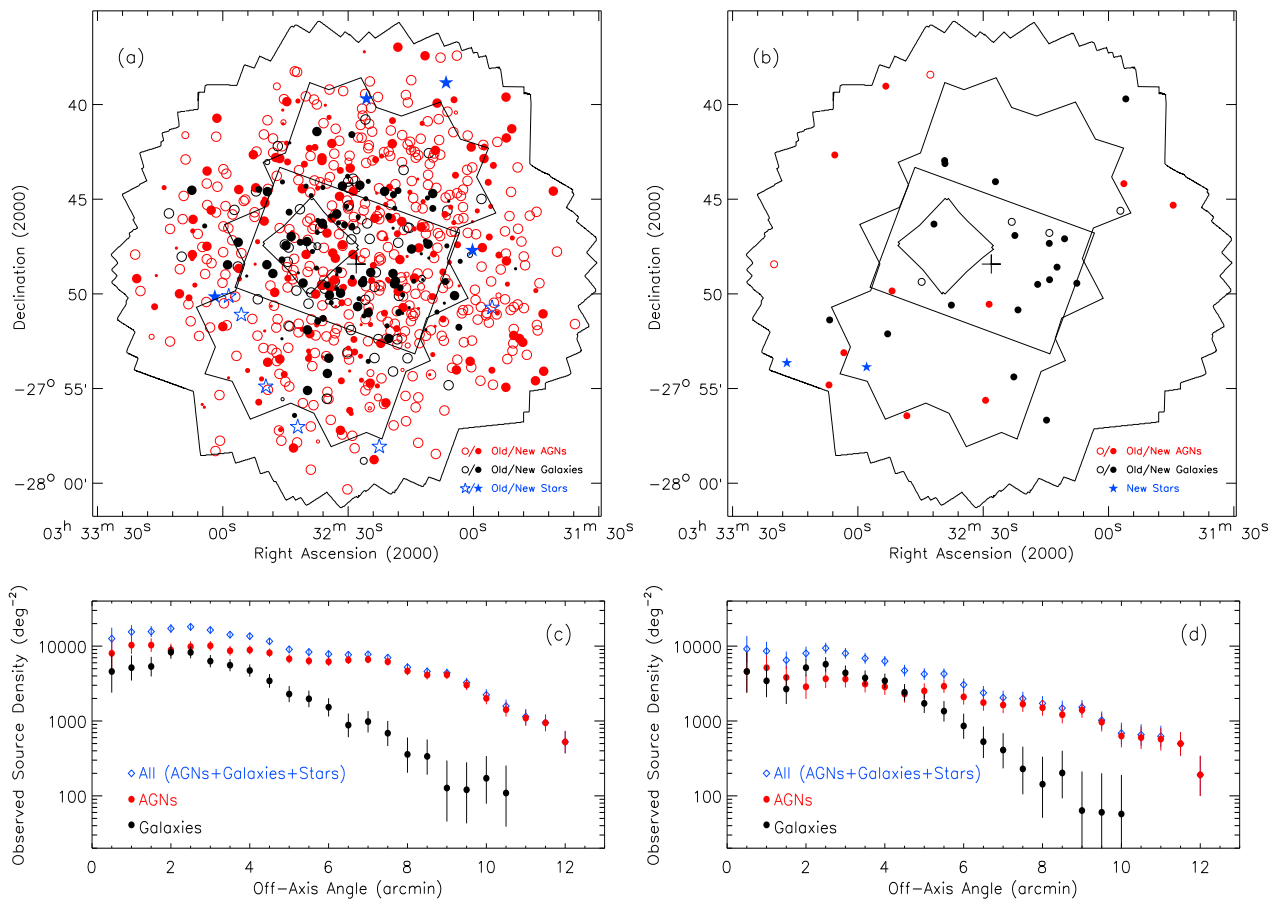
FIG. 13.— (Top) Source spatial distributions for (a) the main catalog and (b) the supplementary optically bright catalog. Sources that are considered AGNs, galaxies, and stars (given in Column 78) are colored red, black, and blue, respectively. Open circles indicate AGNs/galaxies that were previously detected in (a) the L08 main catalog or (b) the L08 main or supplementary optically bright catalog; open stars in (a) indicate stars that were previously detected in the L08 main catalog; filled circles and stars indicate new AGNs/galaxies and stars, respectively. The regions and the plus sign are the same as those in Fig. 1. In panel (a), the sizes of the circles and stars indicate the AE binomial no-source probabilities, with larger sizes indicating lower no-source probabilities: as the size becomes smaller, the AE binomial no-source probability P moves from \log P \leq -5 , -5 < \log P \leq -4 , -4 < \log P \leq -3 , to \log P > -3 . In panel (b), all sources have \log P > -3 and are plotted as circles/stars of the same size. (Bottom) Observed source density for different source types as a function of off-axis angle for (c) all the main-catalog sources and (d) the new main-catalog sources, as computed in bins of \Delta\theta = 1' . 1\sigma errors are calculated using Poisson statistics. [see the electronic edition of the Supplement for a color version of this figure.]
