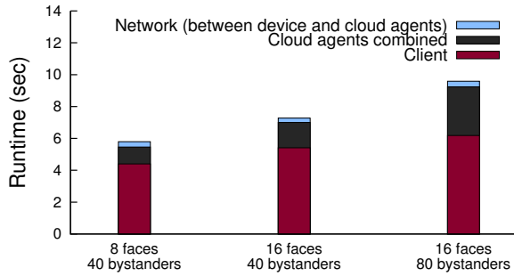
Figure 12. Runtime breakdown of secure matching protocol
