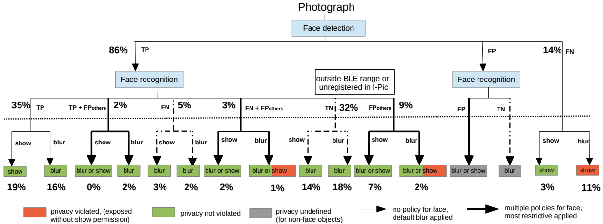
Figure 5. I-Pic decision tree
