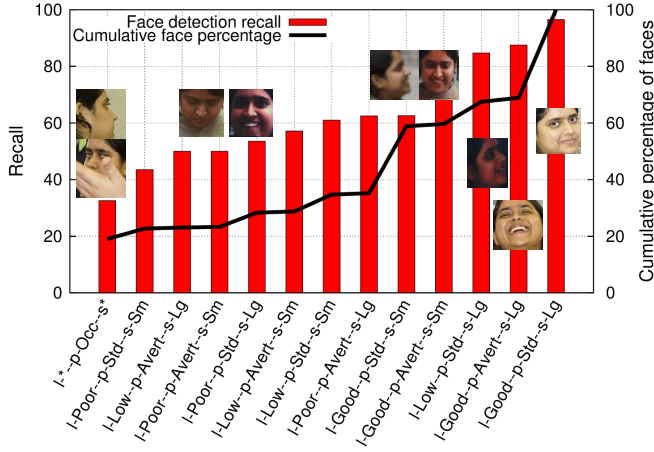
Figure 7. Face detection accuracy vs. illumination conditions, face poses and face sizes
