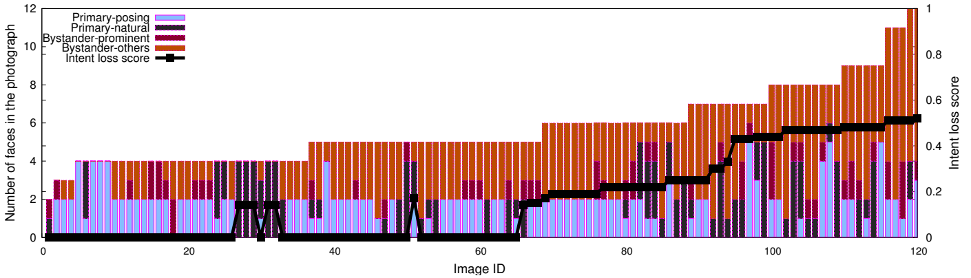
Figure 6. I-Pic Intent score of images
