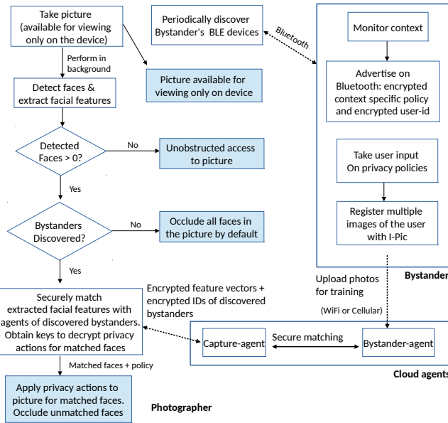
Figure 3. I-Pic workflow
