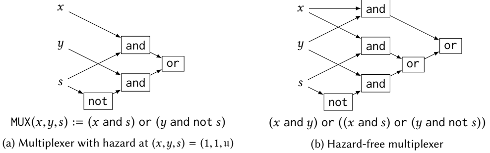
Fig. 1. Two circuits that implement the same Boolean multiplexer function. One has a hazard, the other one is hazard-free.
