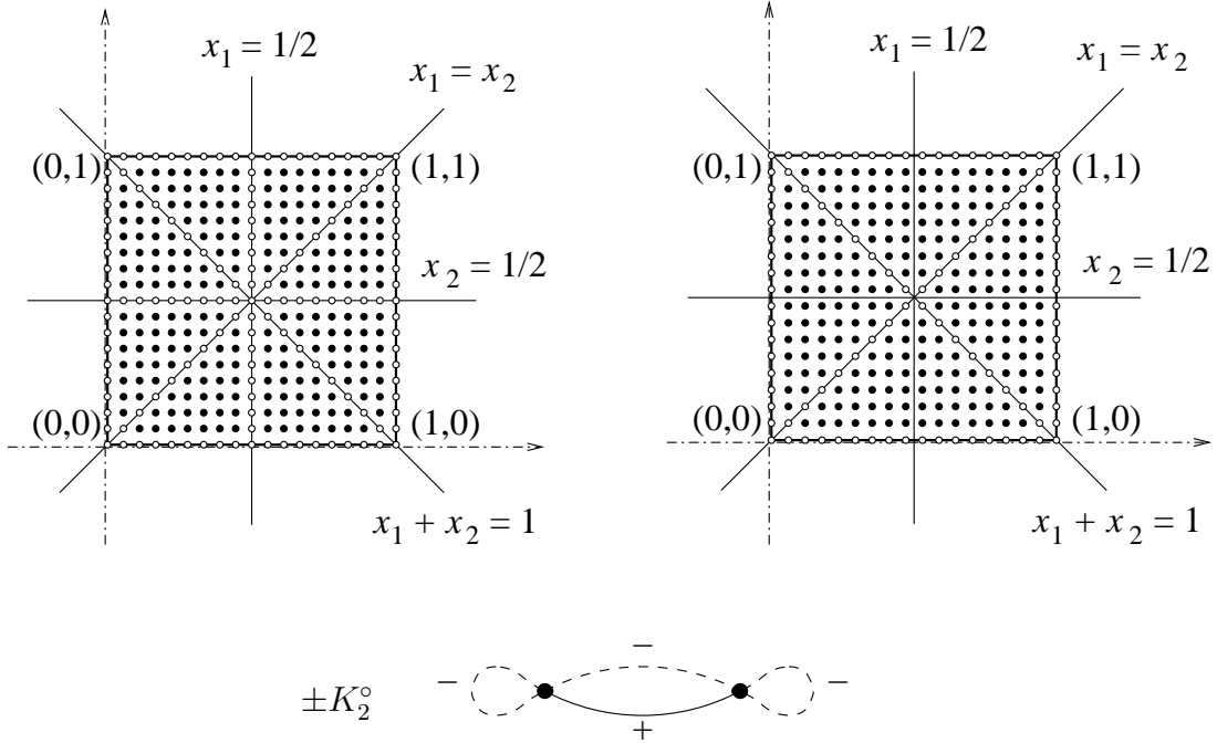
FIGURE 3. Illustrating for k = 8 : On the left, the \frac{1}{2(k+1)} -lattice points in [0, 1]^2 that k -color the signed graph \pm K_2^\circ , with shifted hyperplanes. On the right, the \frac{1}{2k+1} -lattice points that k -color it without 0.
