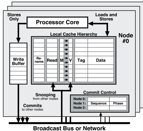
Figure 1: A sample 3-node TCC system.
