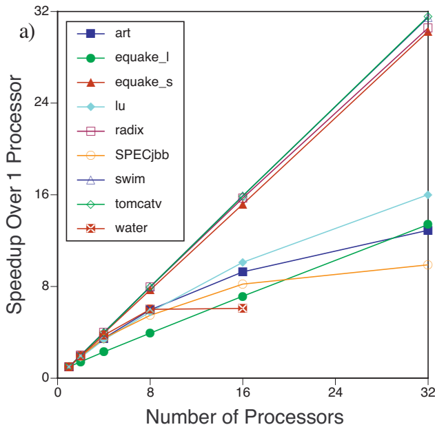
Figure 4: Speedups for varying numbers of processors with our manually parallelized benchmarks (a) and Java benchmarks with automated parallelism (b) on a perfect TCC system with 1 IPC processors, no memory delays, and \infty commit bandwidth.
