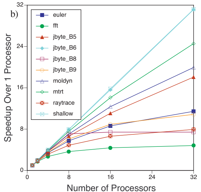
Figure 4: Speedups for varying numbers of processors with our manually parallelized benchmarks (a) and Java benchmarks with automated parallelism (b) on a perfect TCC system with 1 IPC processors, no memory delays, and \infty commit bandwidth.
