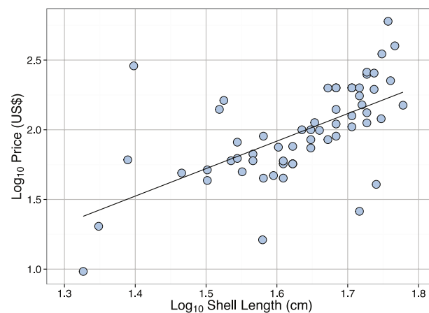
Figure 9 Linear regression between \log_{10} Shell Length (cm) and \log_{10} Price (US$) for Syrinx aruanus . See Table 2 for regression equations.
