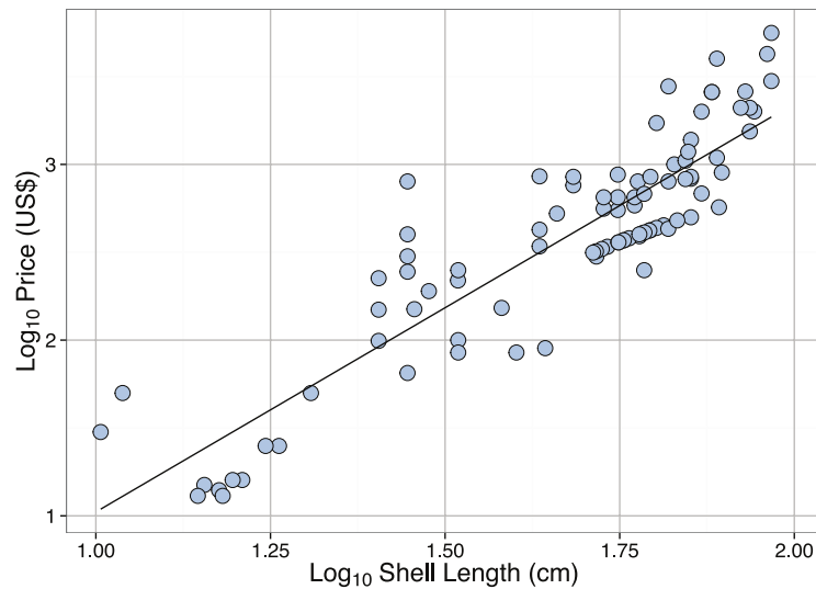
Figure 6 Linear regression between \text{Log}_{10} Shell Length (cm) and \text{Log}_{10} Price (US$) for Tridacna gigas . See Table 2 for regression equations.
