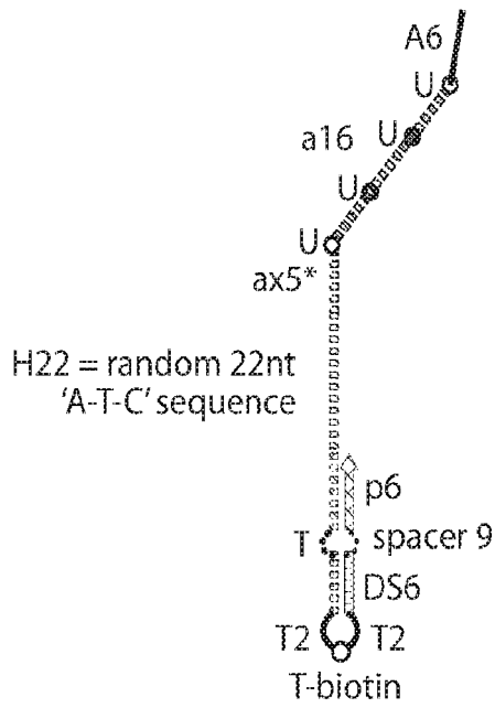
chemically-synthesized probe precursor
