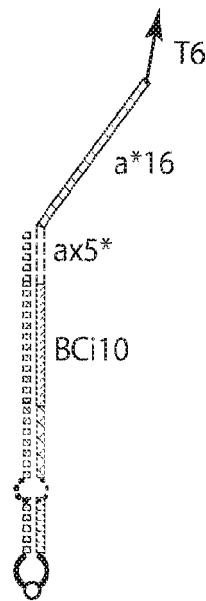
extended precursor 5' end cleaved by 'USER' enzymes (neb.com)
