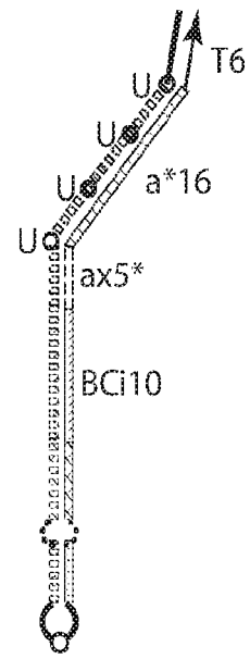
precursor extended by polymerase
