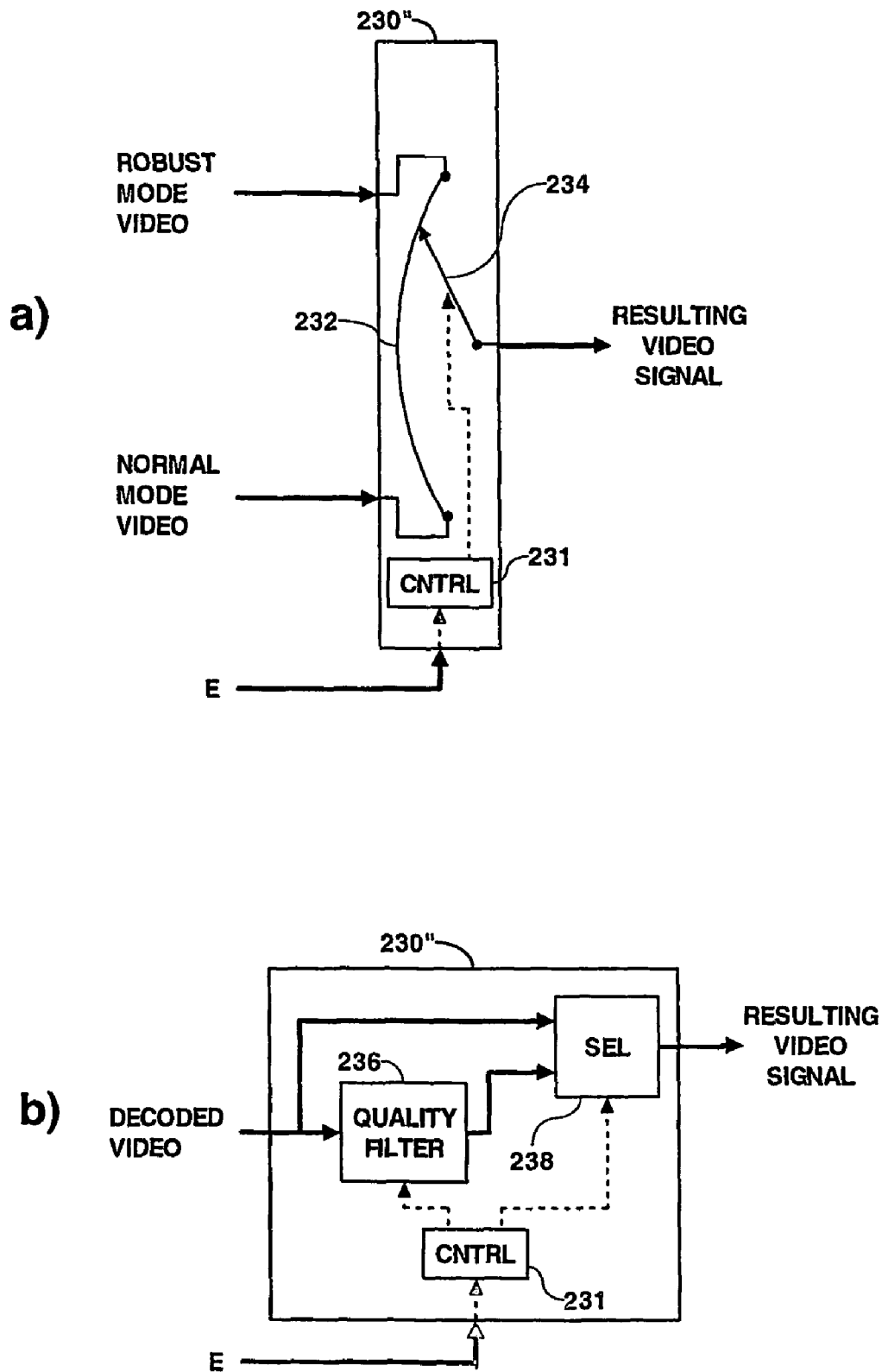
Fig. 5 Smoothing selector
