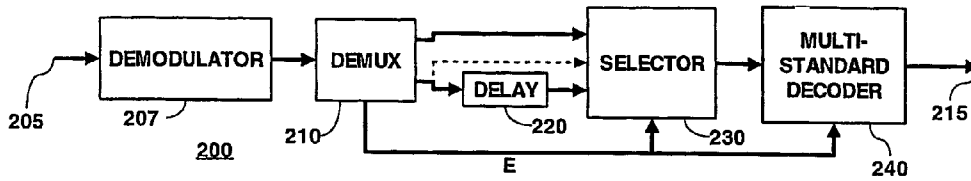
Fig. 2 Receiver
