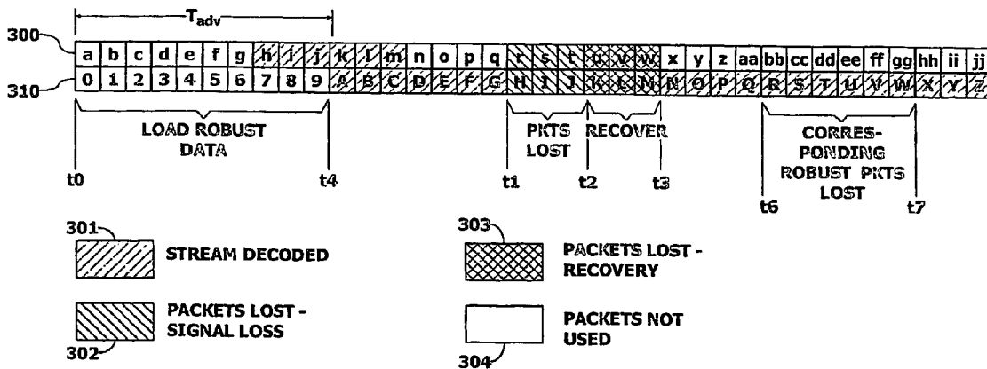
Fig. 3 Packet Streams
