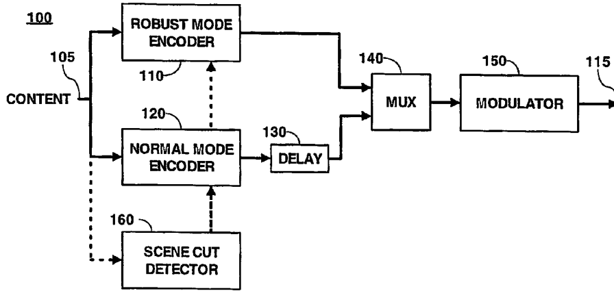
Fig. 1 Transmitter
