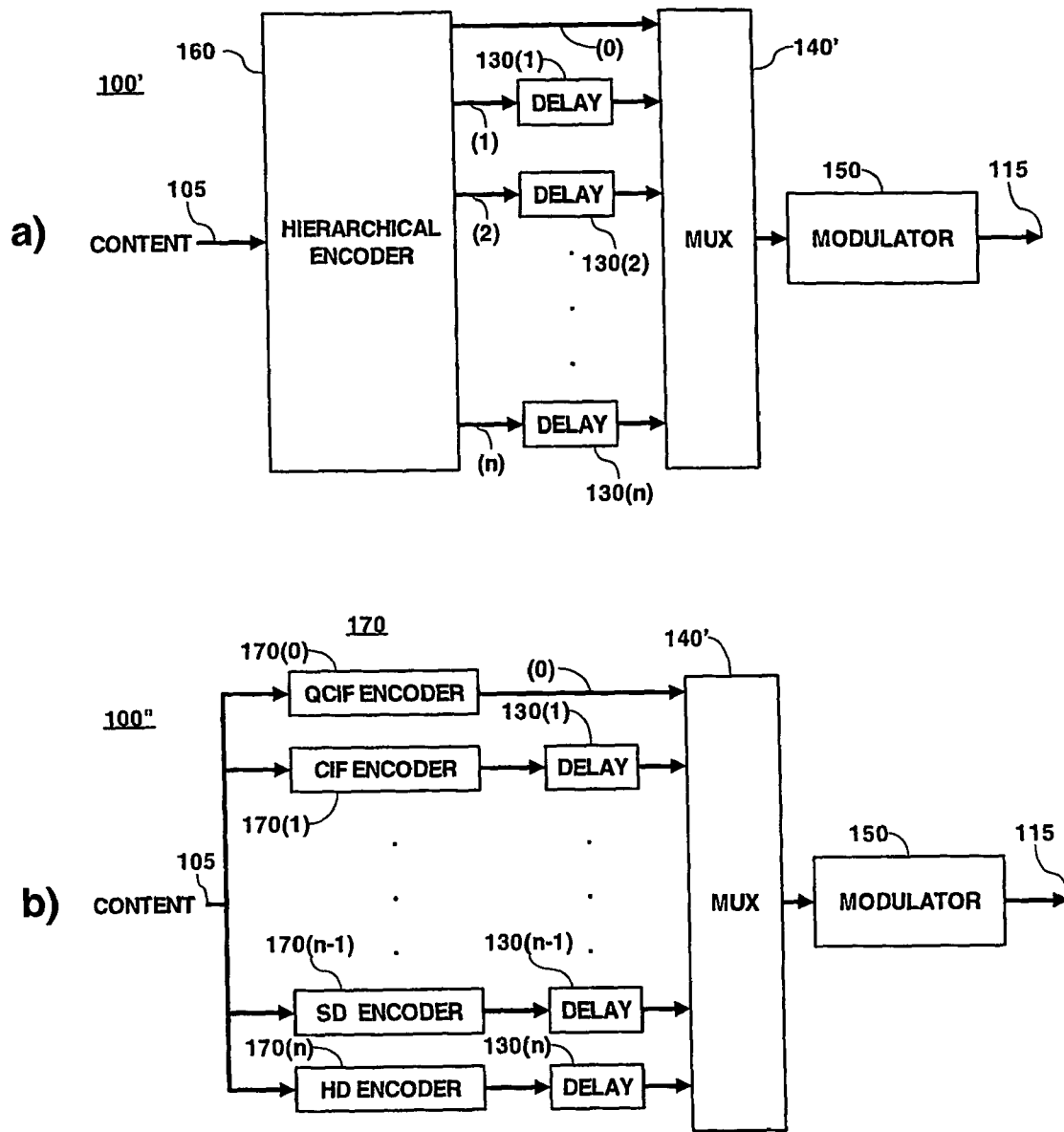
Fig. 9 Multiresolution transmitter
