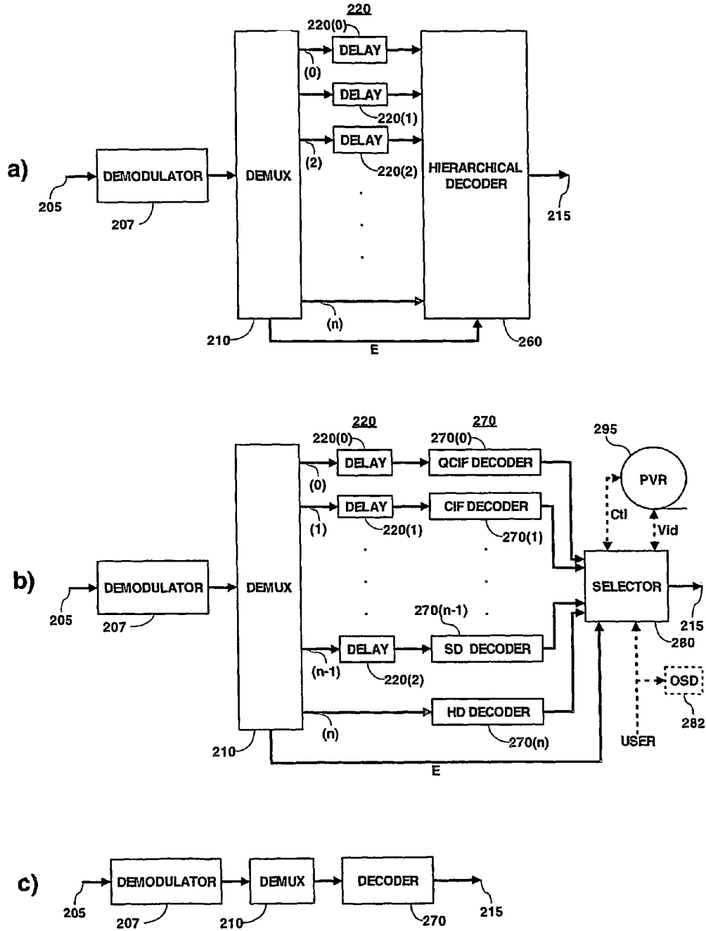
Fig. 10 Multiresolution receiver
