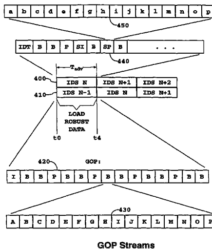
GOP Streams
