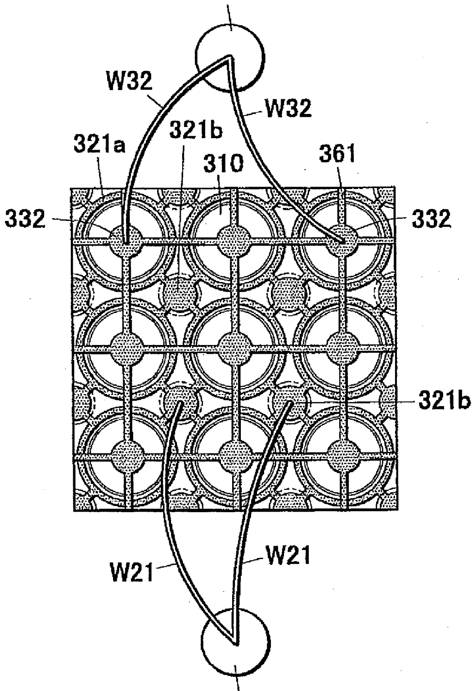
Negative Side Terminal T2
