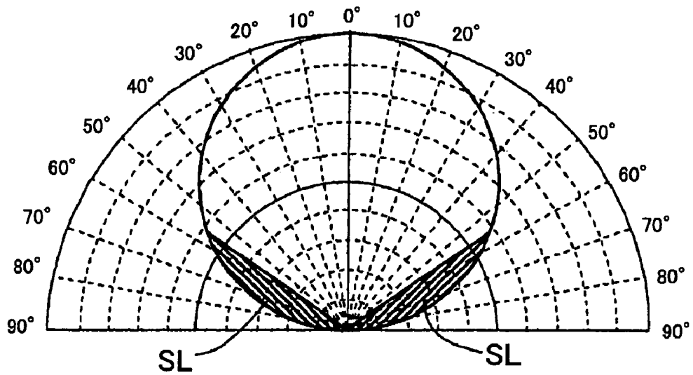
Directivity characteristic of light source
