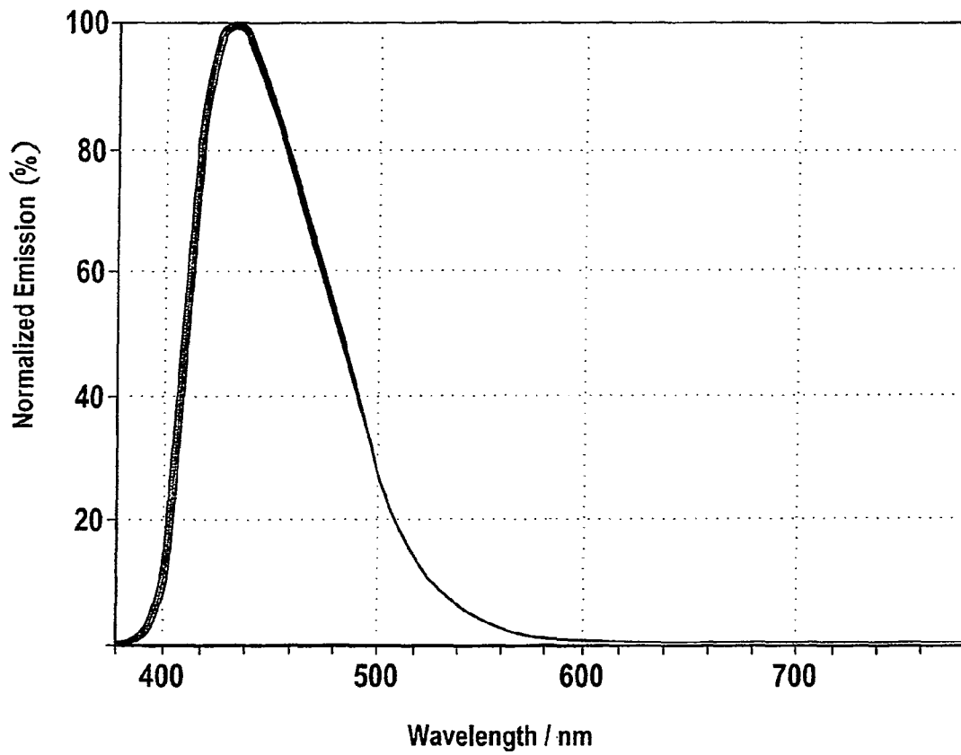
Spectral Graph (Relative Spectral Distribution)
