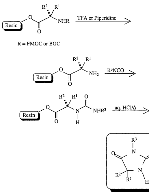
SCHEME 2
