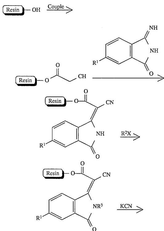
SCHEME 12
