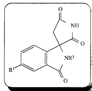
SCHEME 13
