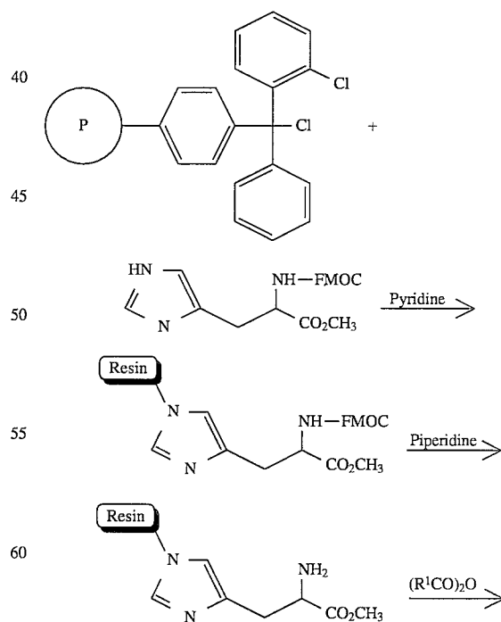
SCHEME 13
