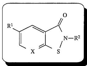
SCHEME 12
