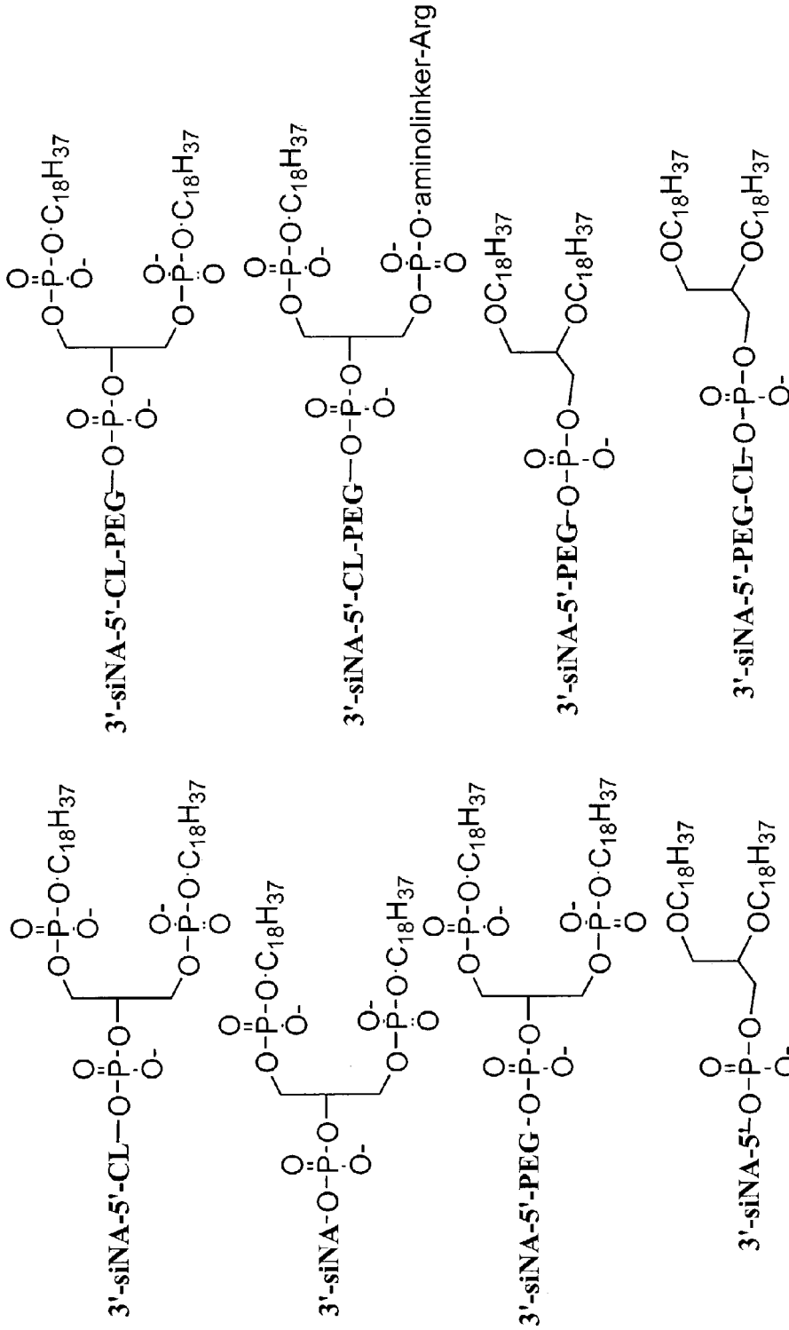
Figure 51: siNA/Phospholipid Conjugates
