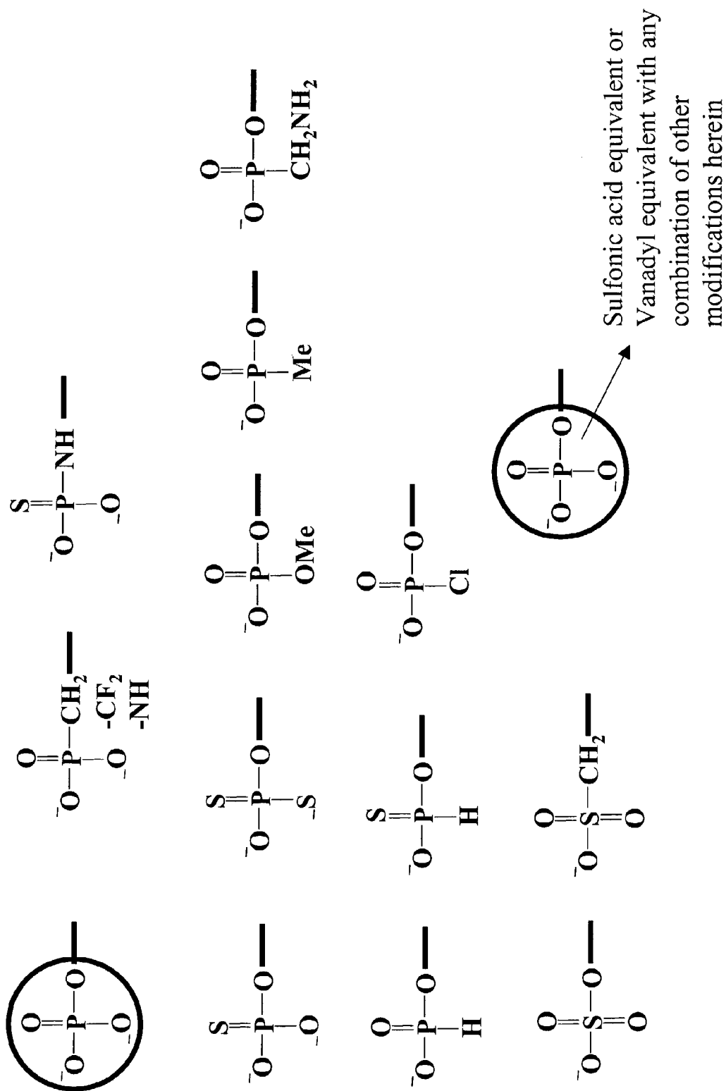
Figure 75: 5'-phosphate modifications
