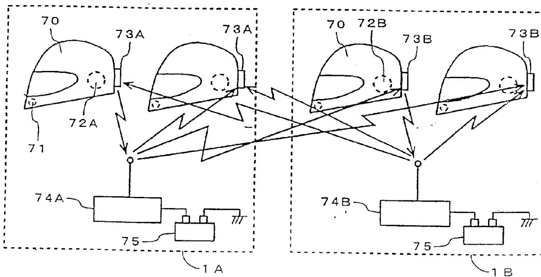
74A, 74B: REPEATING APPARATUS
