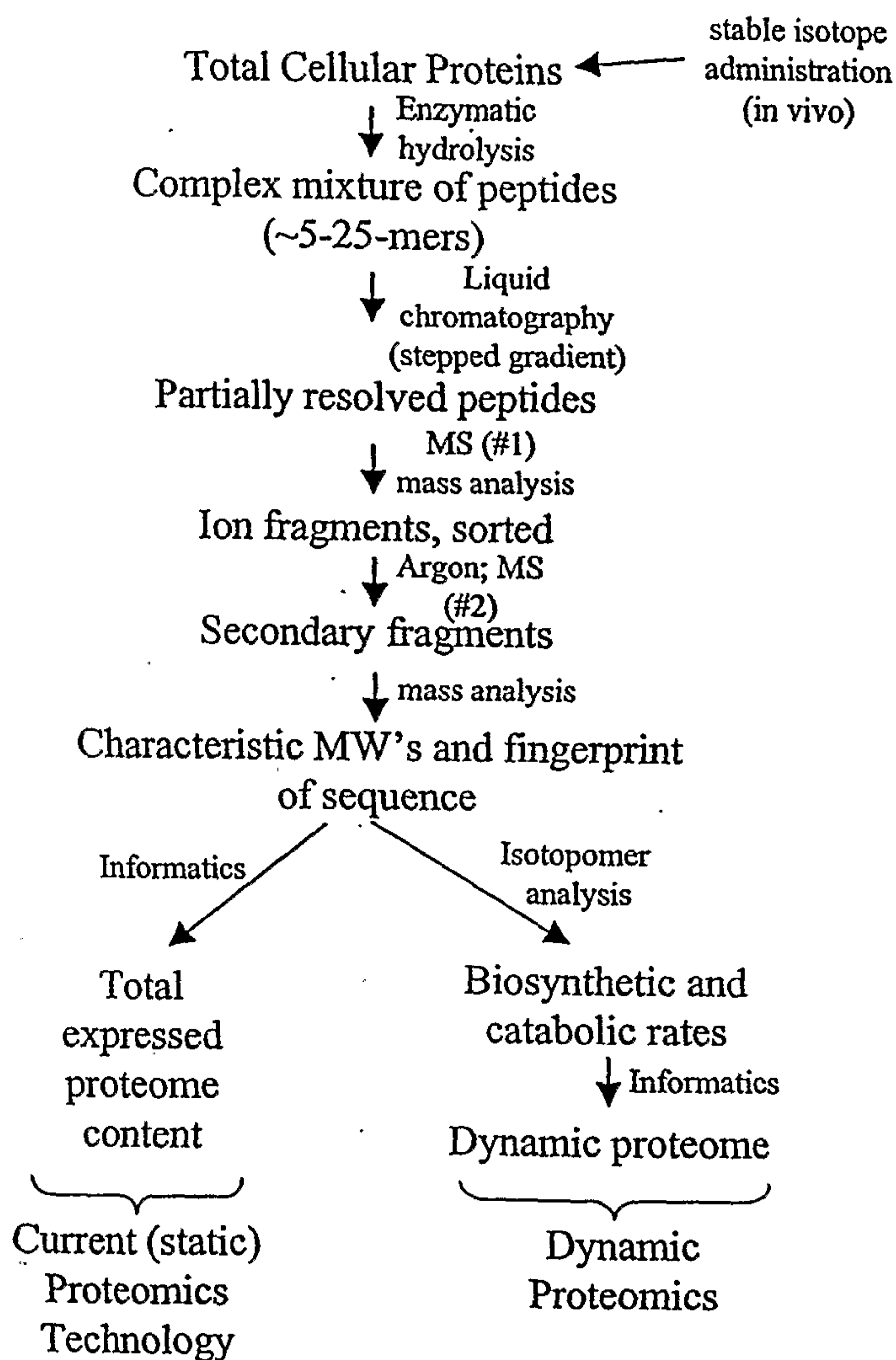
Fig. 3. Technique for Measuring Dynamic Proteomics
