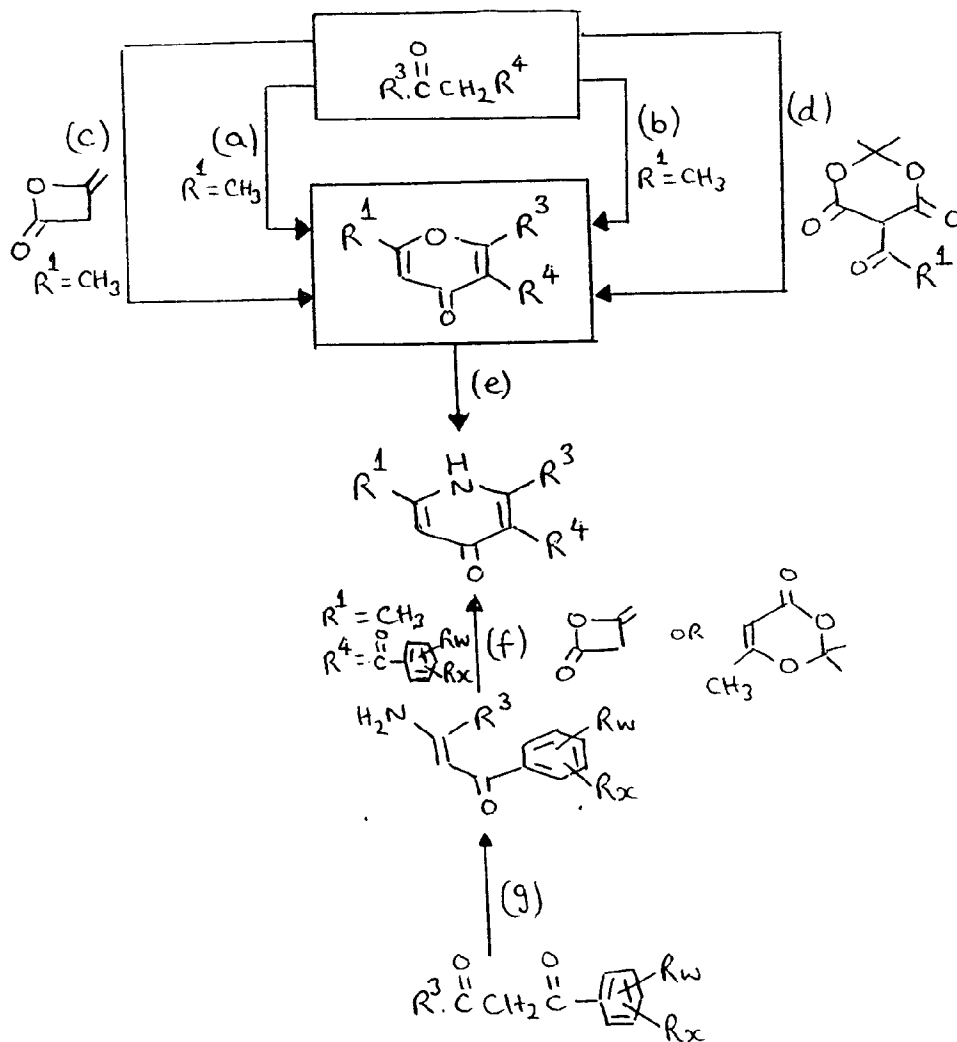
Scheme 3
