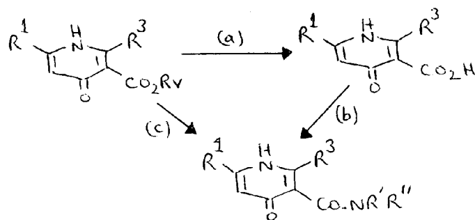
Scheme 5
