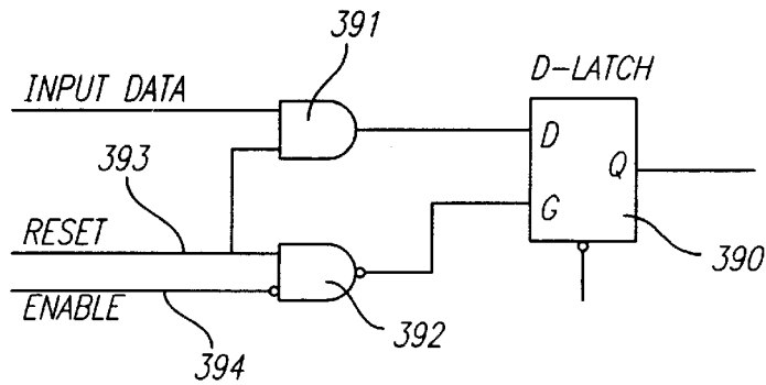
FIG. 37 FAILING IMPLEMENTATION OF A LATCH WITH CLEAR
