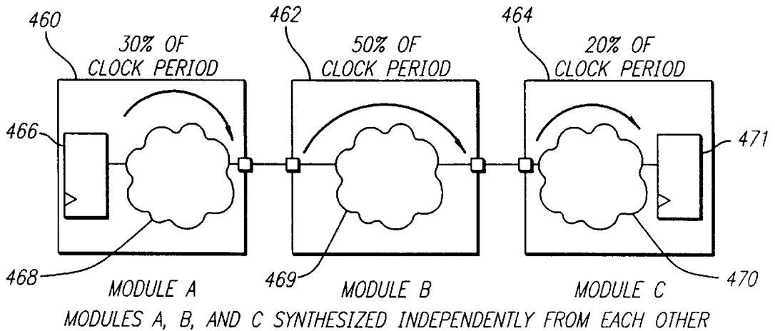
FIG. 20C TIME BUDGETS
