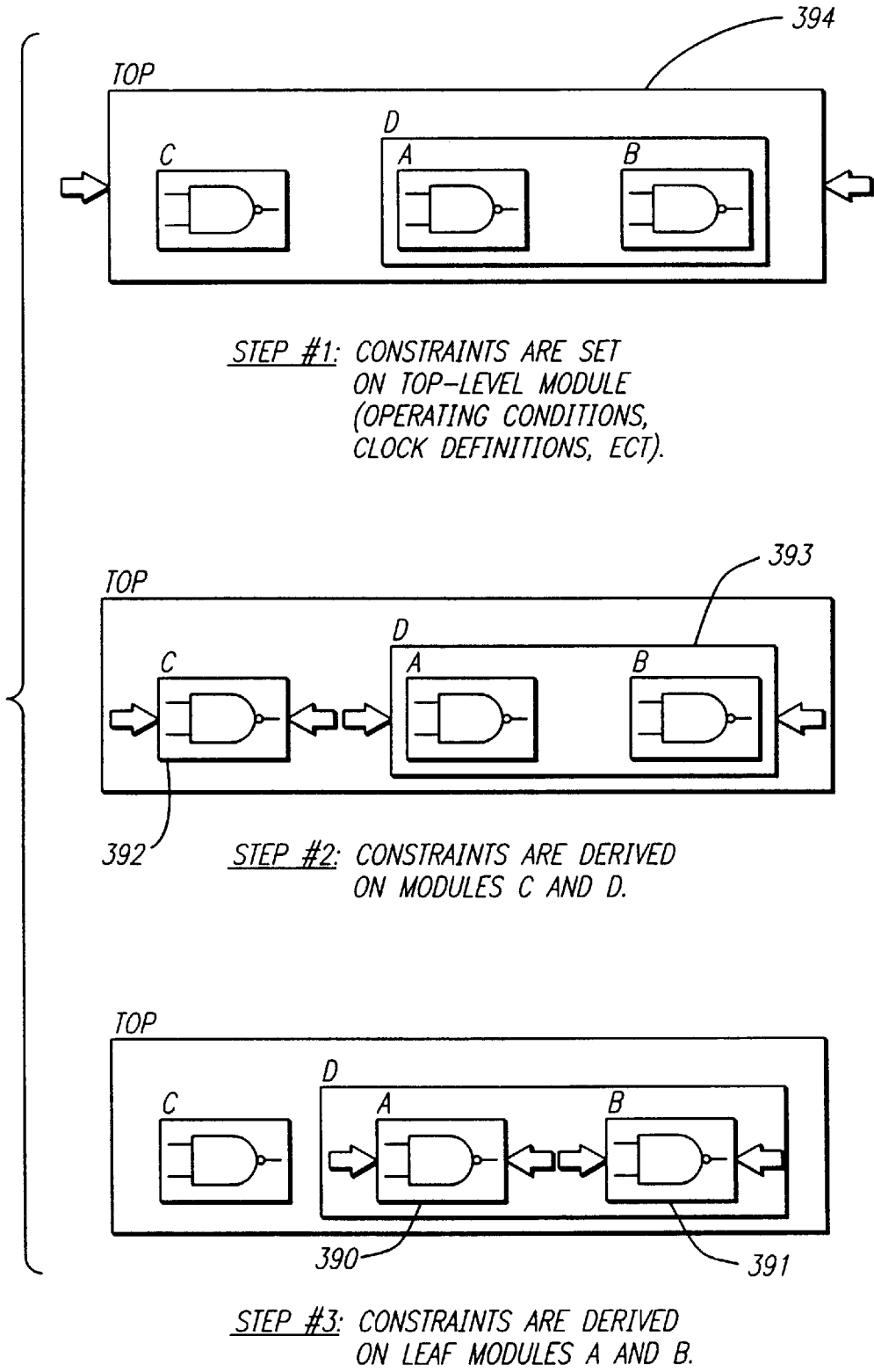
FIG. 16 TOP-DOWN CHARACTERIZATION
