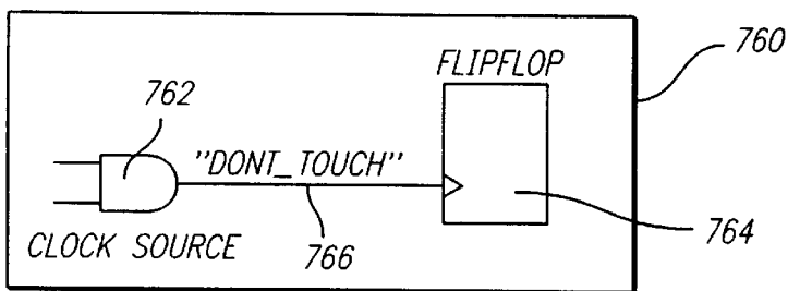
FIG. 41C CLOCK SOURCE RETRIEVED THROUGH USING THE CONNECTED NET. RETRIEVING NAMES OF NEW SOURCE PINS.
