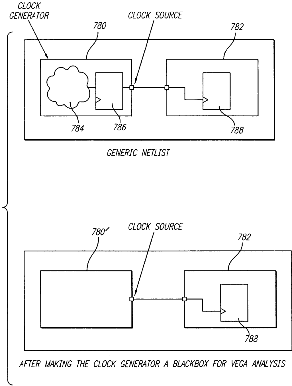
FIG. 43 HANDLING CLOCK GENERATORS WITH A "BACKBOX_DESIGN" DIRECTIVE.
