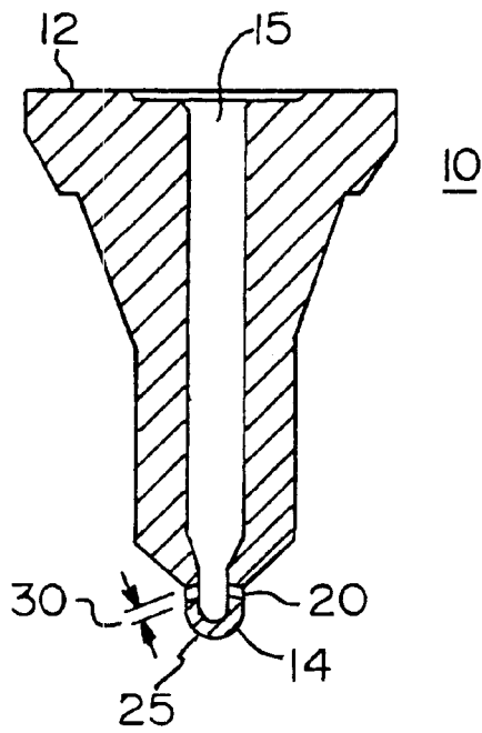
FIG. 2 PRIOR ART
