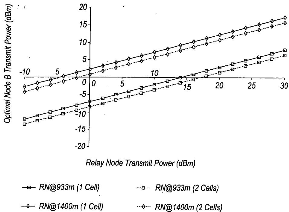
Optimal NB transmit power as a function of RN transmit power for a non-regenerative relay for TDD for each deployment scenario where it is assumed the NB to UE link has a 3dB gain compared with the other links.
