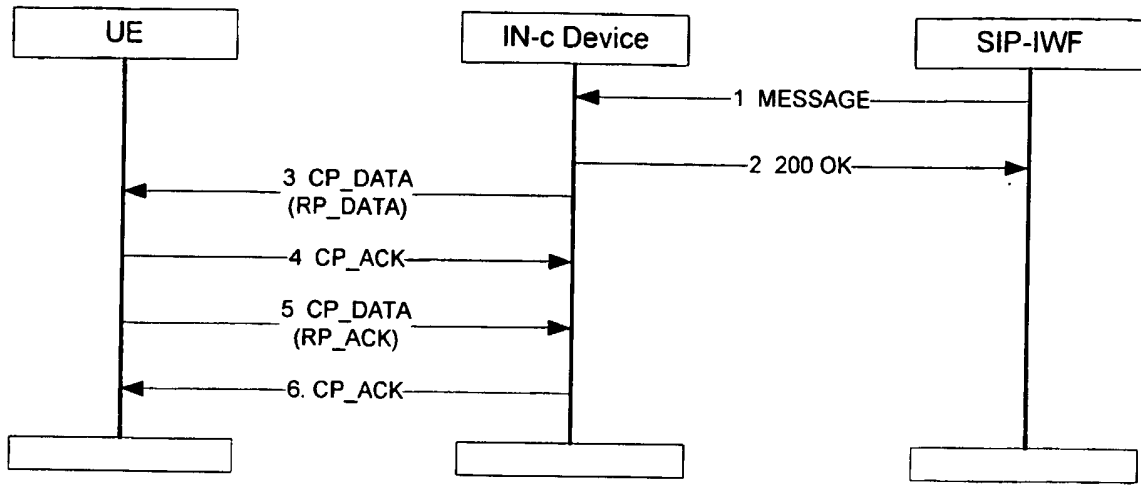
Figure 45: MT SMS Transfer
