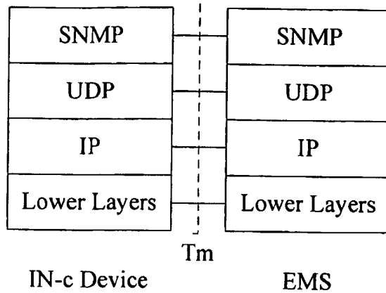
Figure 8: Control Plane IN-c Device – EMS
