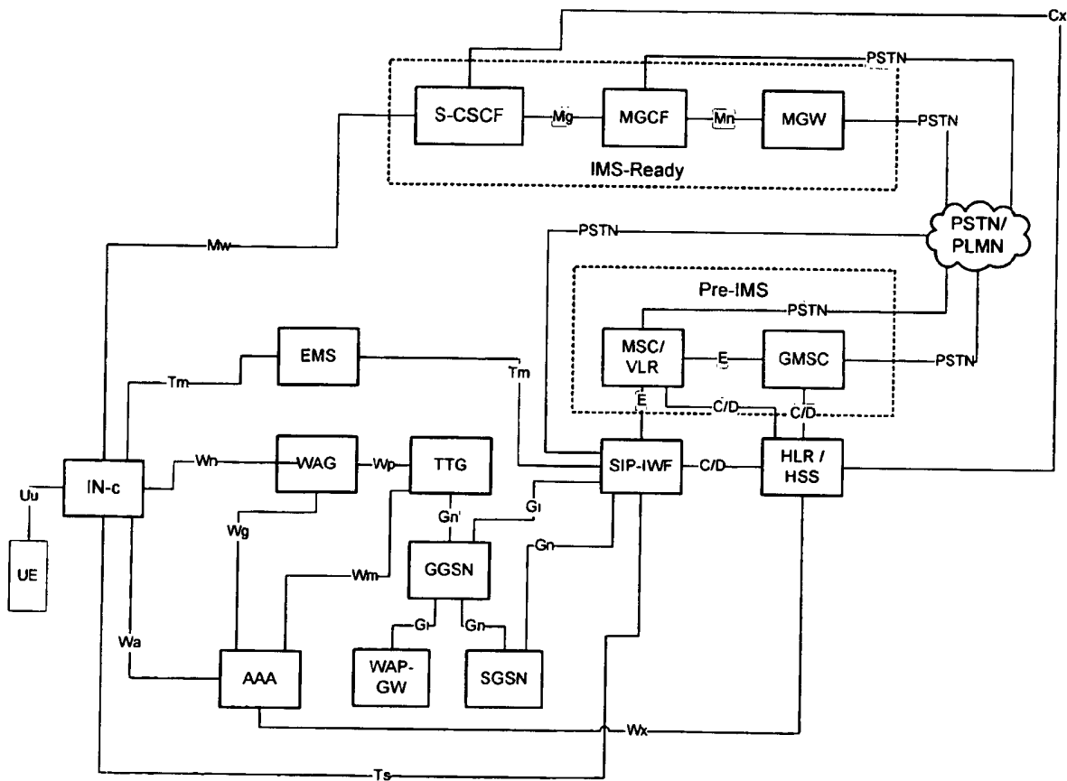
Figure 2 Logical Architecture for IN-c Network
