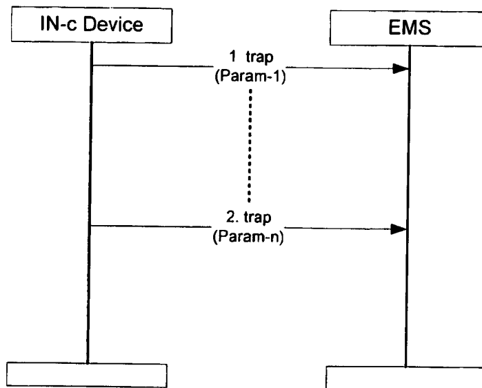
Figure 48: Error and Event Reporting in IN-c Device
