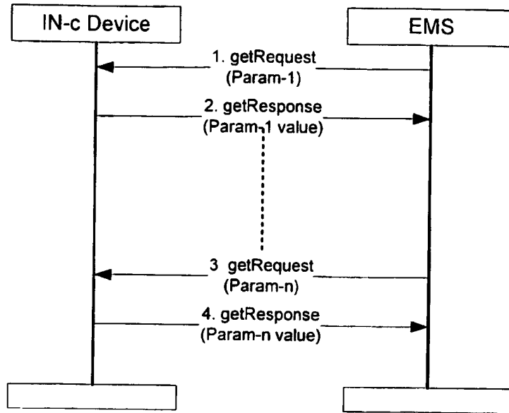
Figure 47: EMS Auditing the IN-c Device
