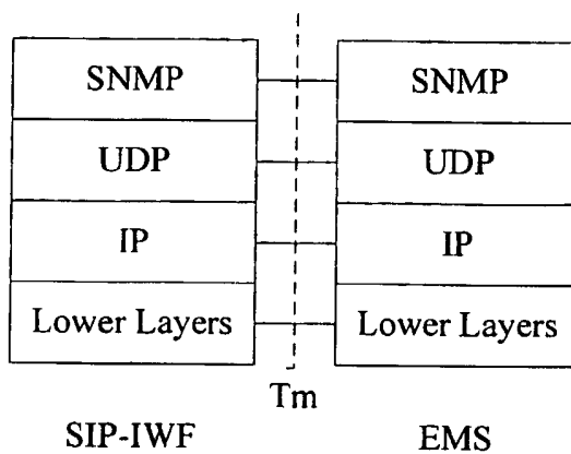
Figure 10: Control Plane SIP-IWF – EMS
