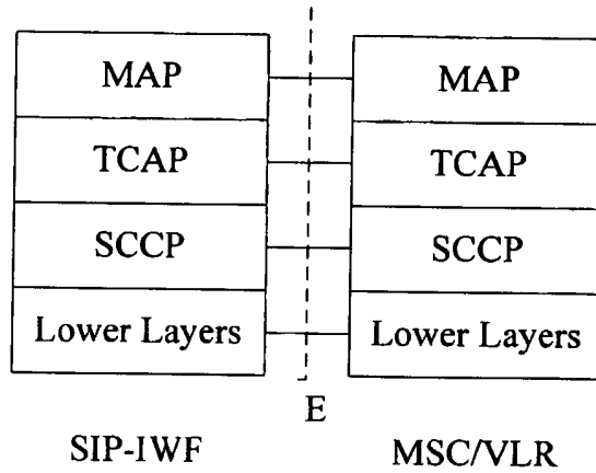
Figure 12: Control Plane SIP-IWF – MSC/VLR
