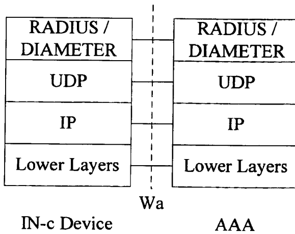
Figure 9: Control Plane IN-c Device – AAA Server
