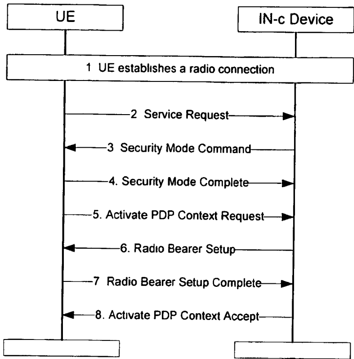
Figure 43: Packet Access to Internet
