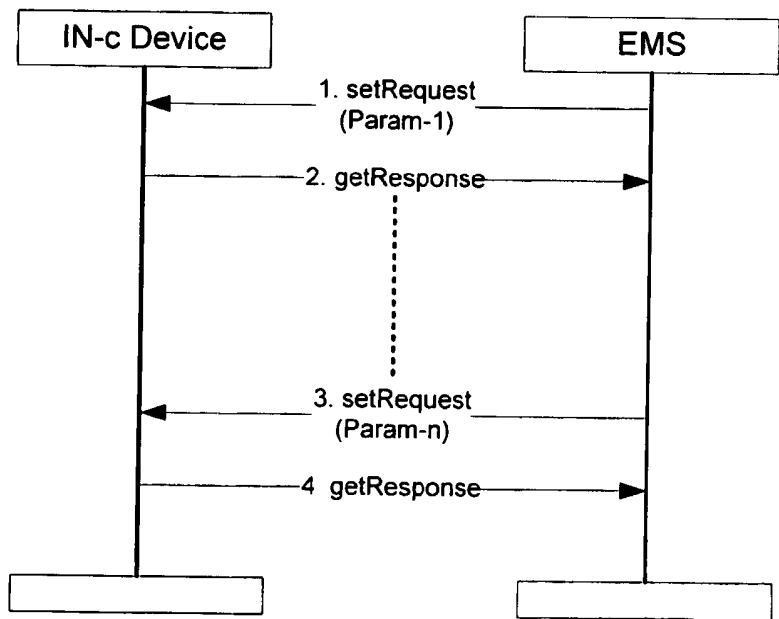
Figure 46: EMS Configuring IN-c Device
