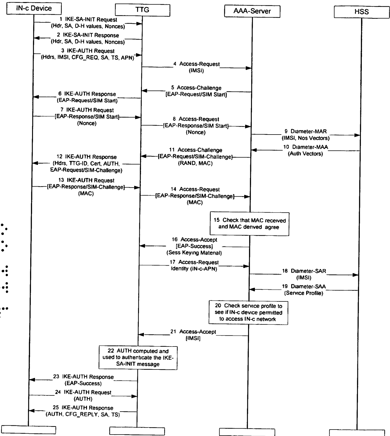
Figure 34: IPsec Tunnel Establishment from IN-c Device to TTG using Radius and EAP-SIM
