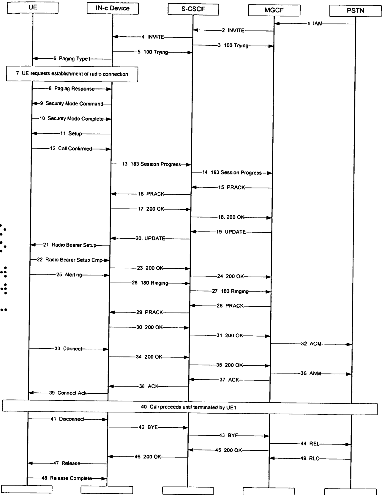
Figure 41: MT CS Voice Call Originating in the PSTN - IMS-Ready Network
