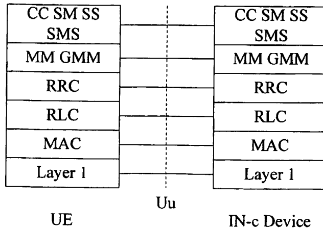
Figure 5: Control Plane UE – IN-c Device
