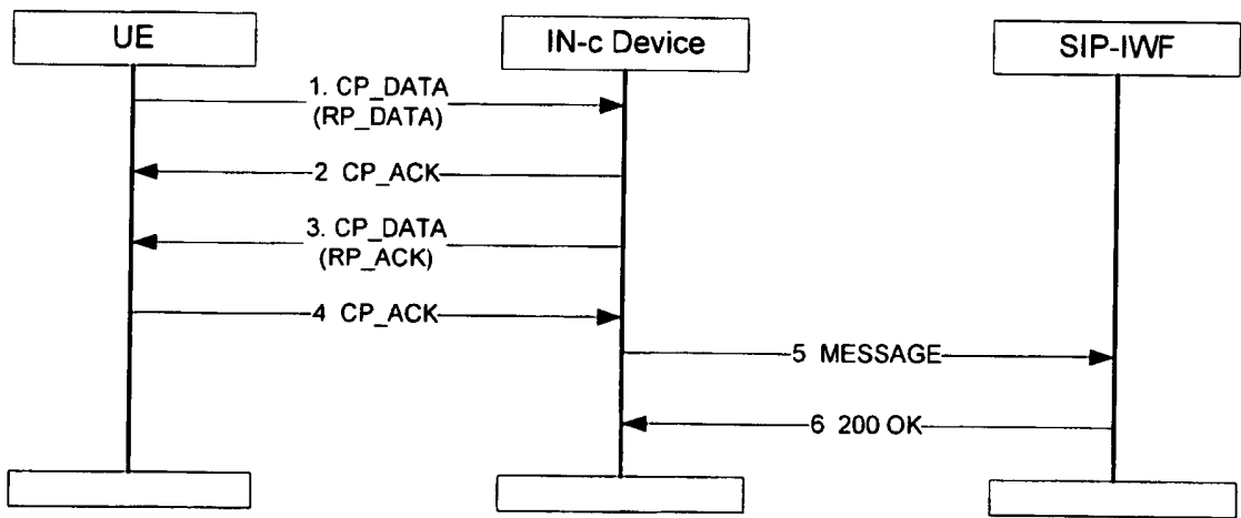
Figure 44: MO SMS Transfer
