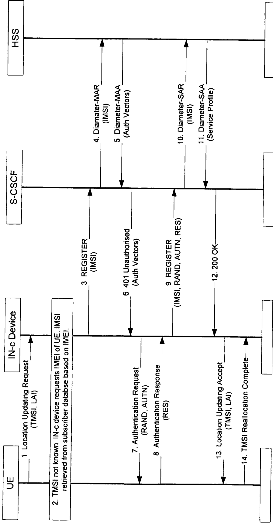
Figure 29: IMS Registration – TMSI Not Known
