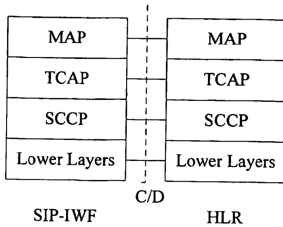
Figure 11: Control Plane SIP-IWF – HLR
