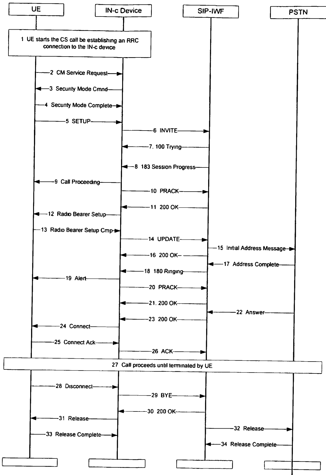
Figure 36 MO CS Voice call terminating in the PSTN – Pre IMS Network
