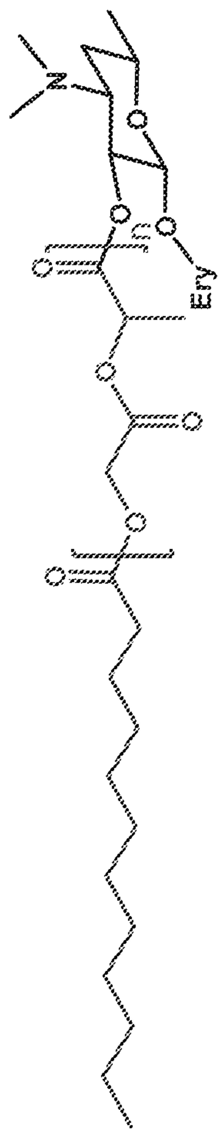
Lauric-PLGA-Erythromycin conjugate
