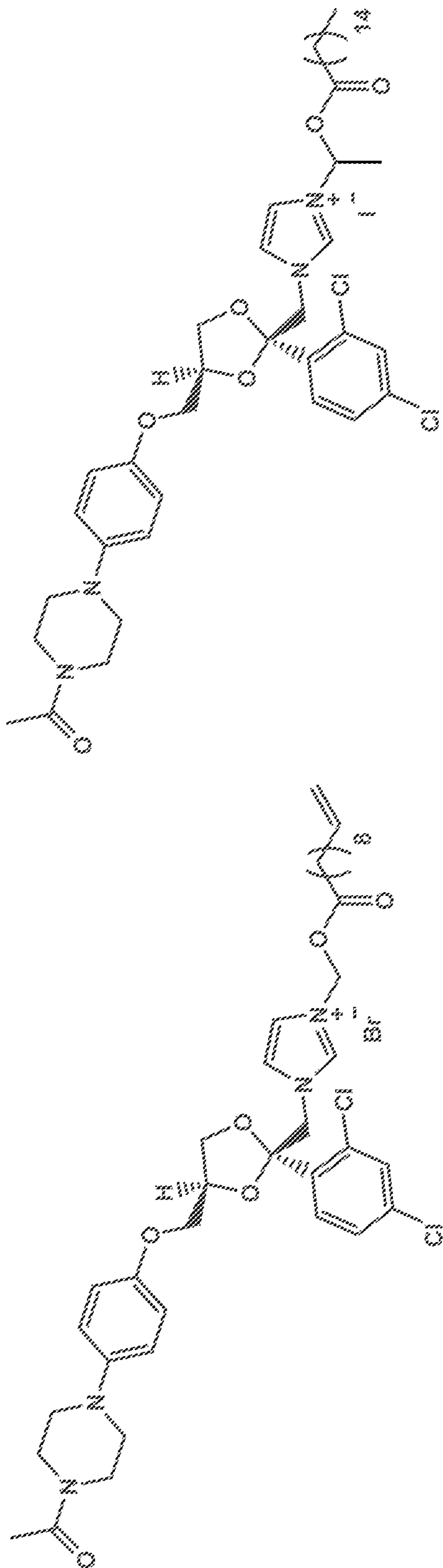
Ketoconazole-methylene-10-undecylenate conjugate
