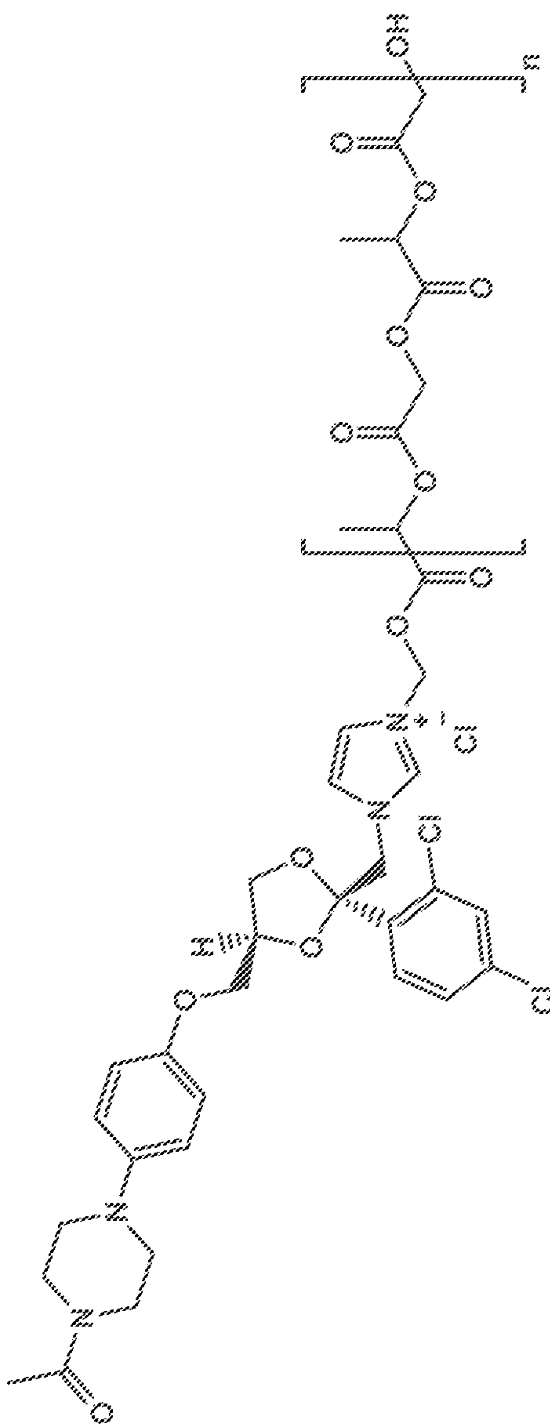
Ketoconazole-methylene-10-undecylenate conjugate
