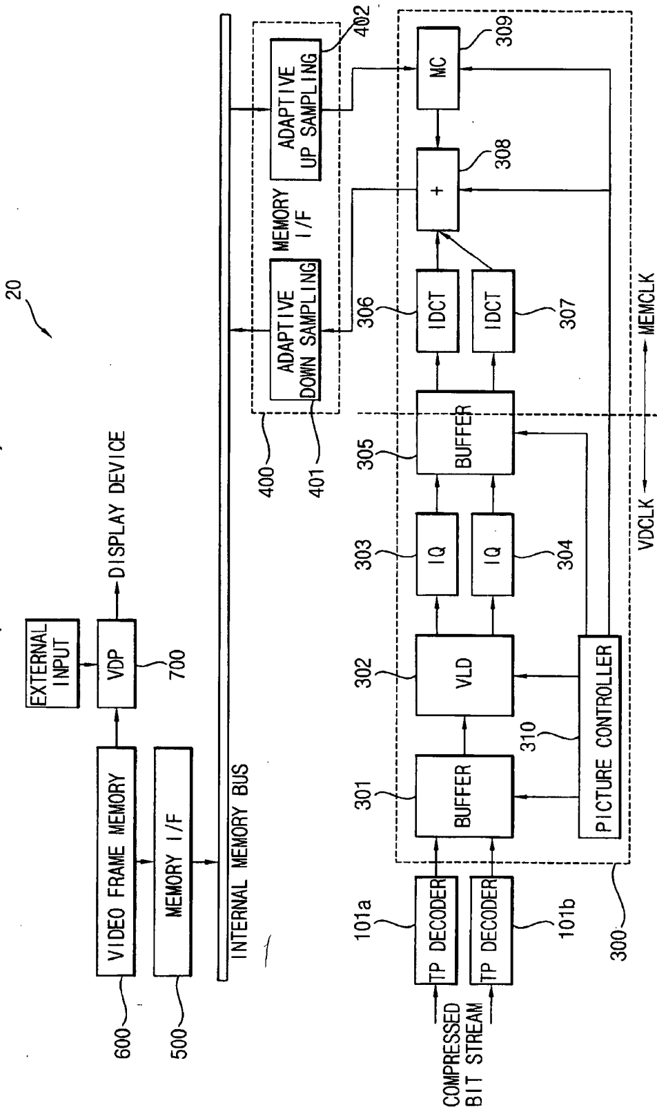
FIG. 2 (PRIOR ART)
