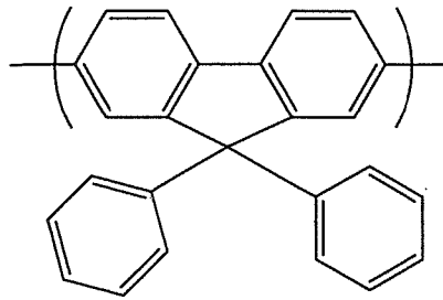
"DPF"
