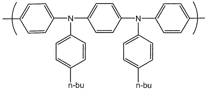
"n-bu PFB"
