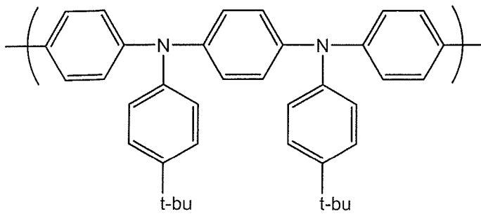
"t-bu PFB"
