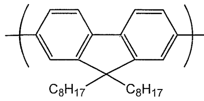
"F8"
