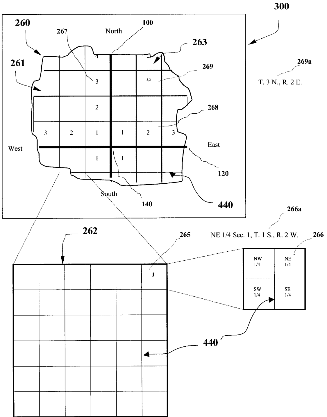
Fig. 2 Prior Art - Public Land Survey System (PLSS)
