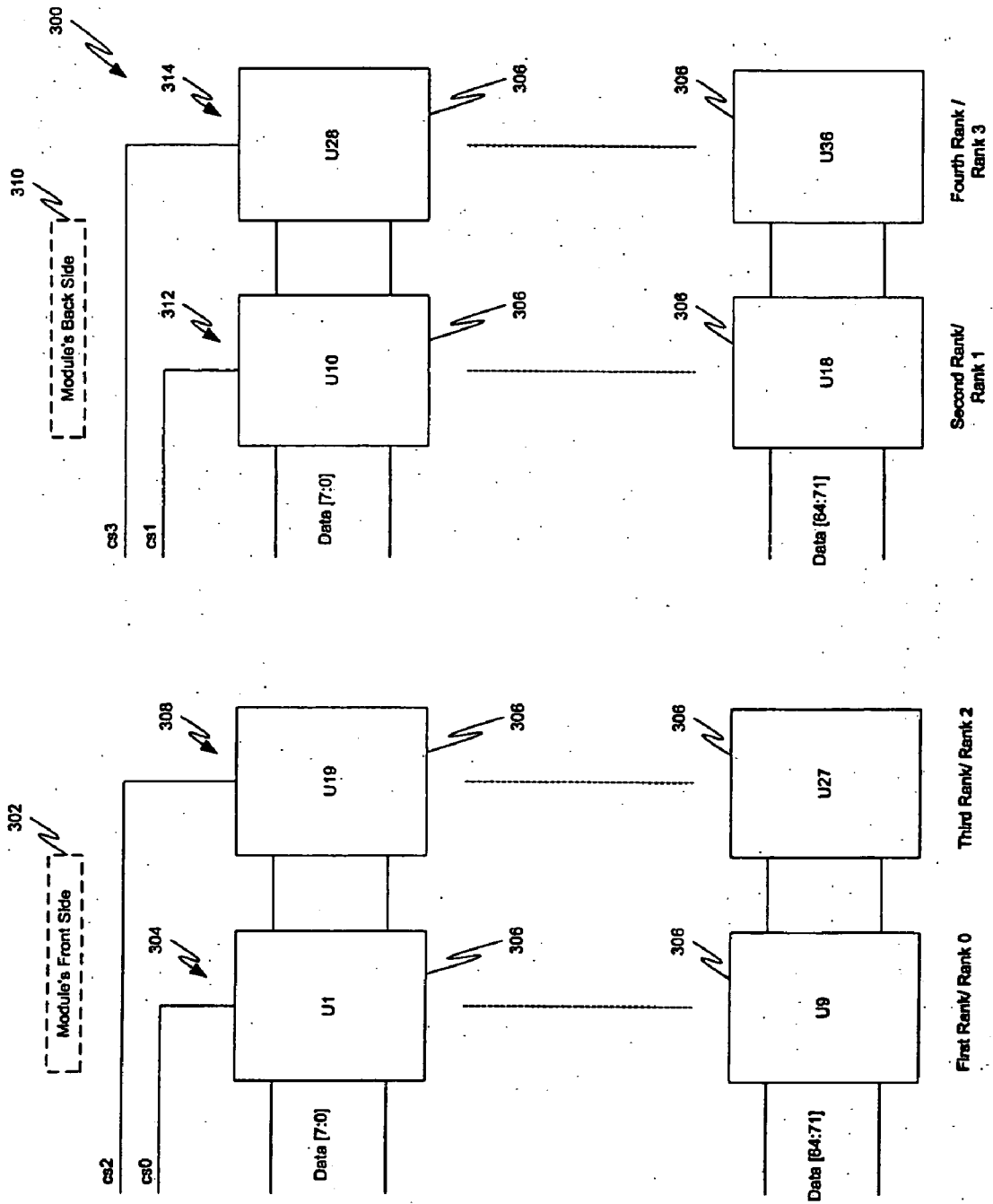
Transparent Four Rank DDR Module Block Diagram
