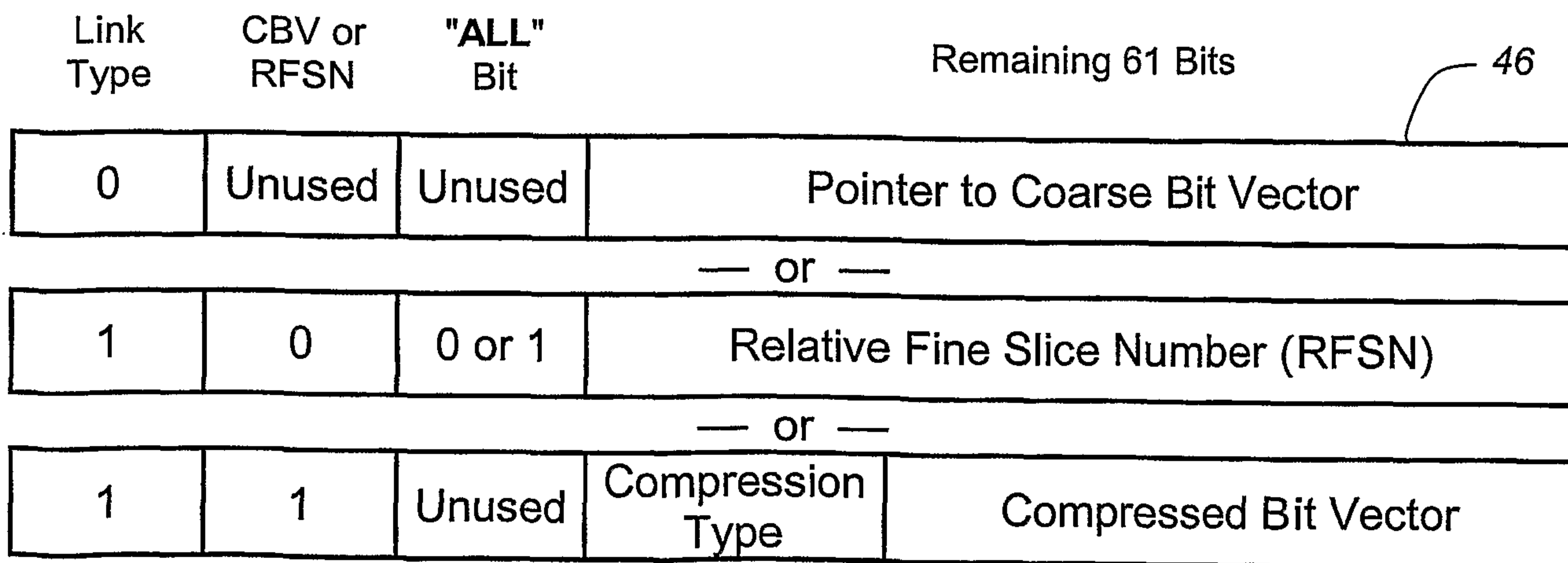
Coarse Link Layout
