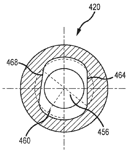
SECTION E-E
