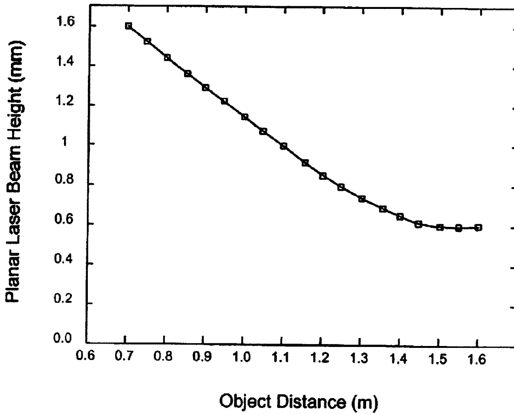
Planar Laser Beam Height vs. Object Distance (Far Object Distance Focus)
