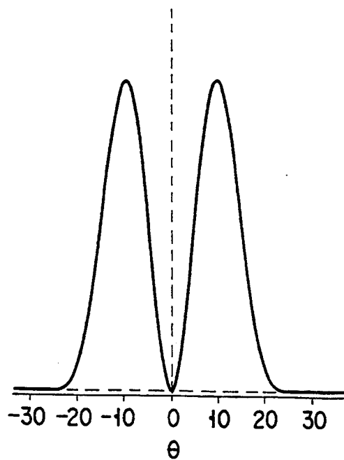
LP11 MODE
