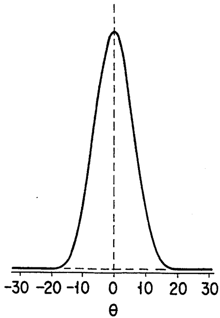
LP01 MODE
