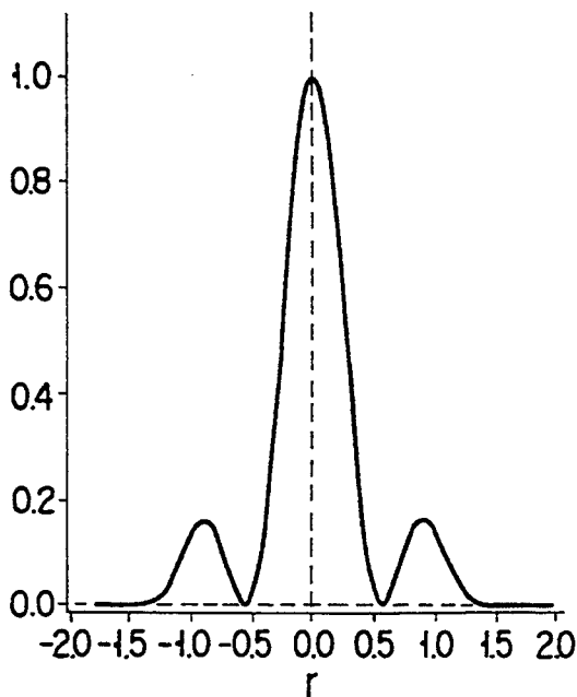
LP02 MODE
