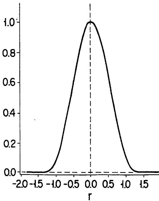
LP01 MODE
