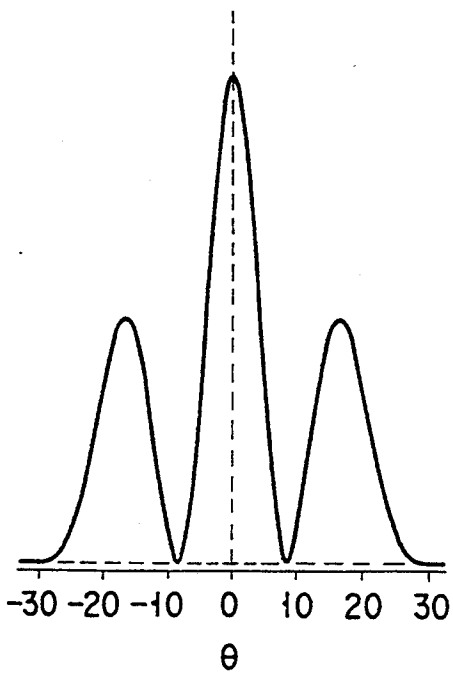
LP02 MODE
