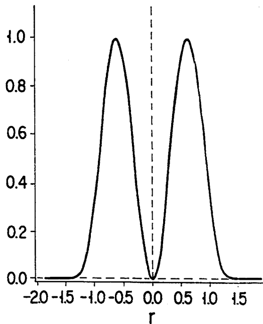
LP11 MODE
