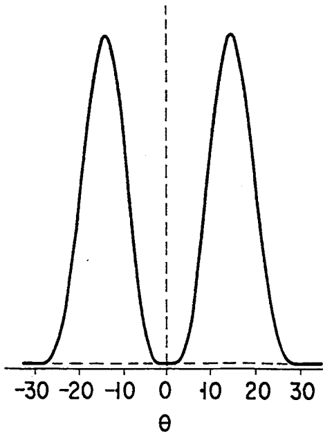
LP21 MODE
