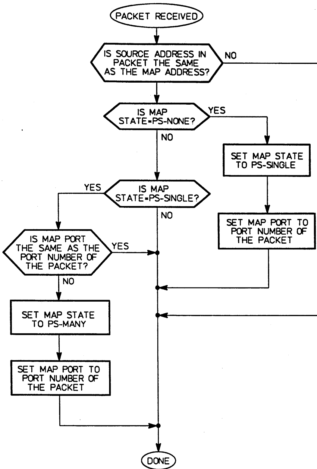
MAPPING ADDRESS SEARCH-HUB IMPLEMENTATION
