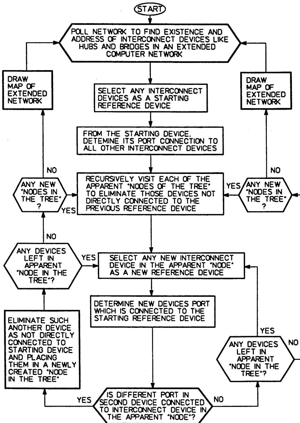
PHYSICAL TOPOLOGY FLOW CHART
