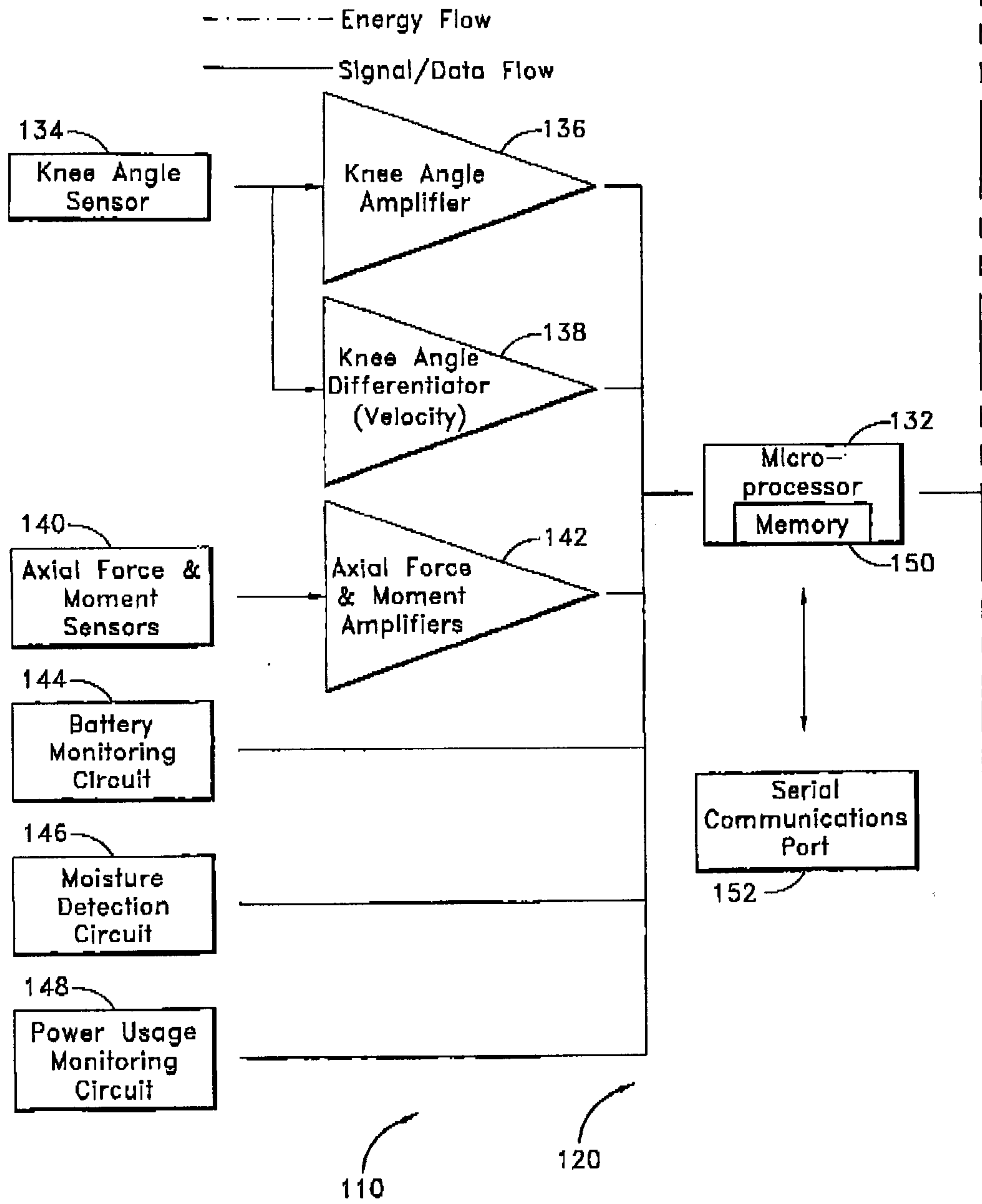
Knee Electronics Block Diagram
