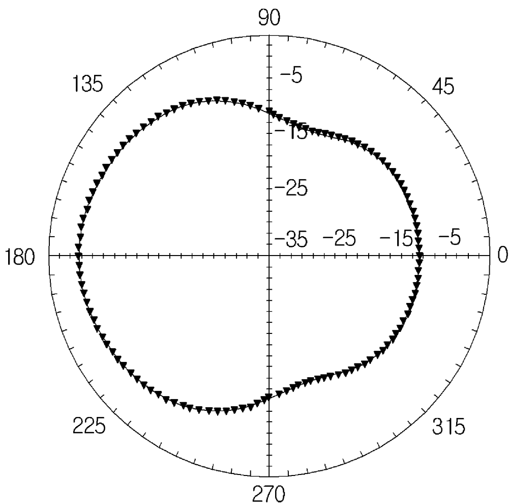
2.4GHz Pattern
