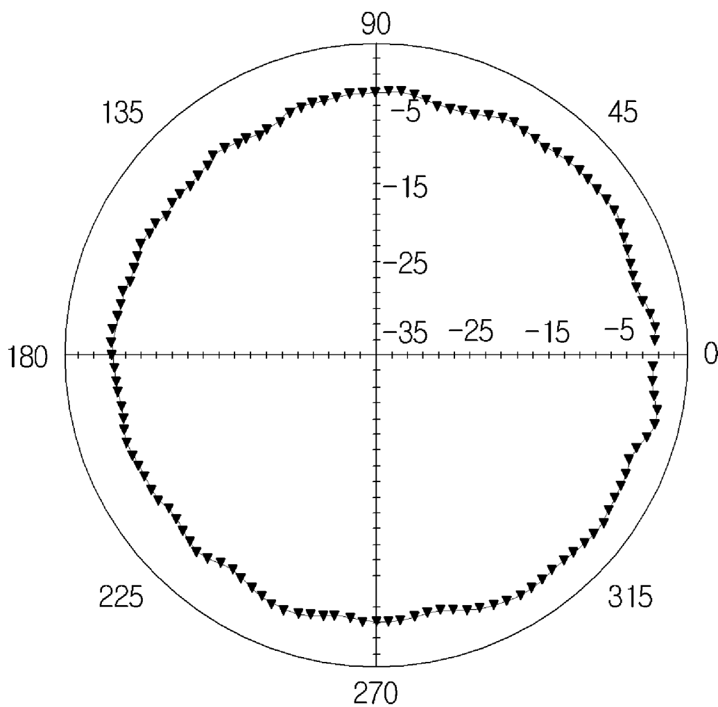
3.5GHz Pattern
