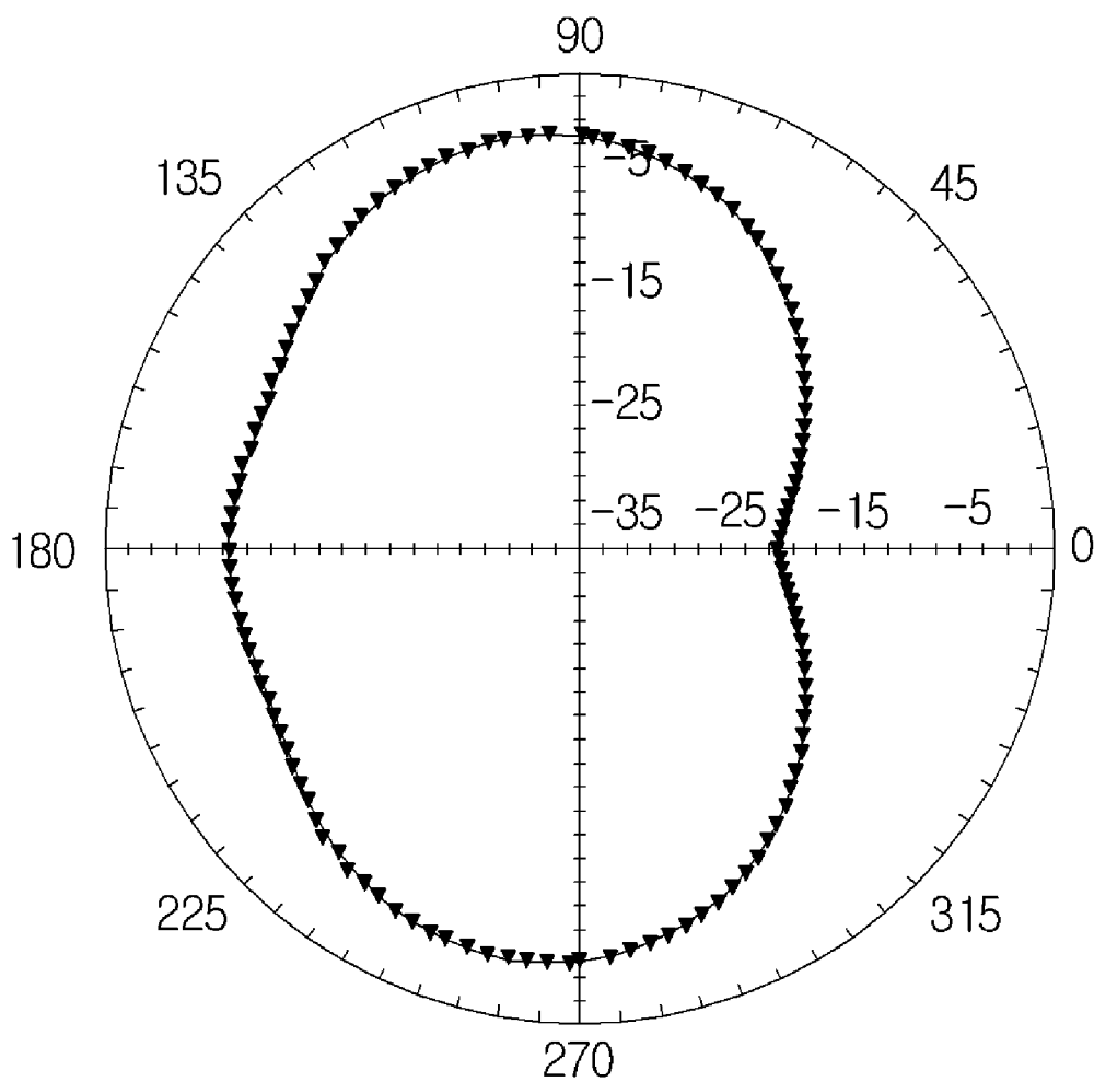
5.55GHz Pattern
