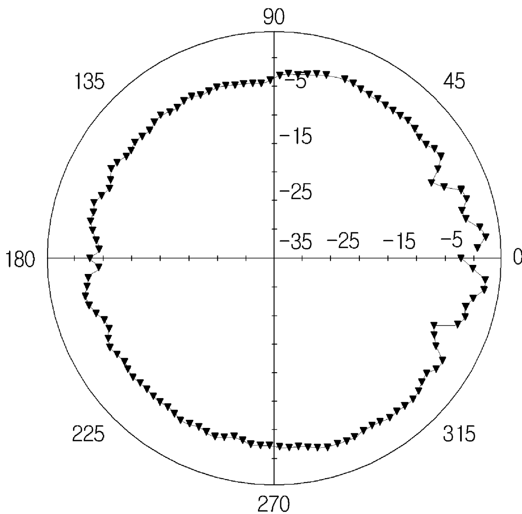
2.4GHz Pattern
