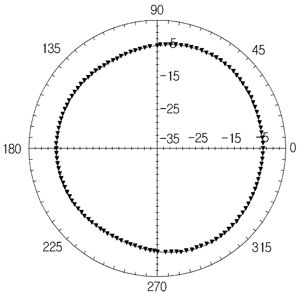
3.5GHz Pattern
