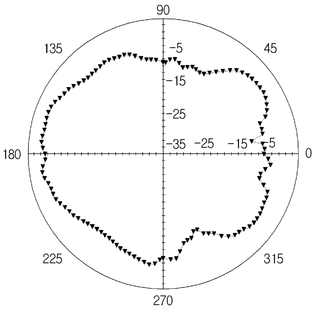
5.55GHz Pattern
