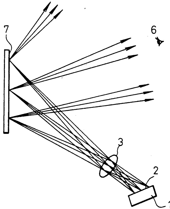
Fig. 28 (PRIOR ART)
