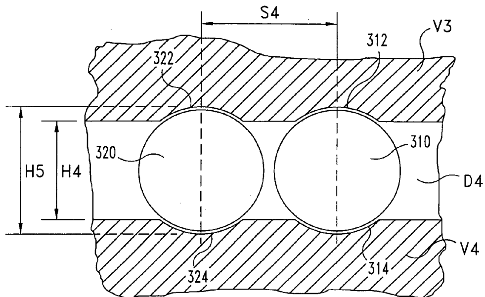
Fig. 11 (PRIOR ART)
