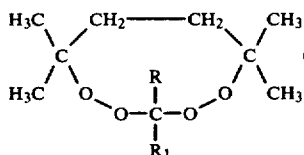
6,6,9,9-Tetramethyl-3R-3R 1 -1,2,4,5-Tetraoxycyclononane
