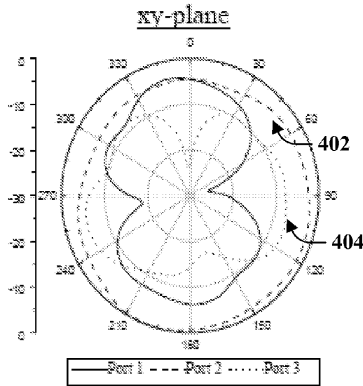
Fig. 4. Measured far-field patterns of the 3-port tri-polarized dipole antenna at 2.58 GHz.
