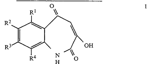
CHEMICAL FORMULAE
