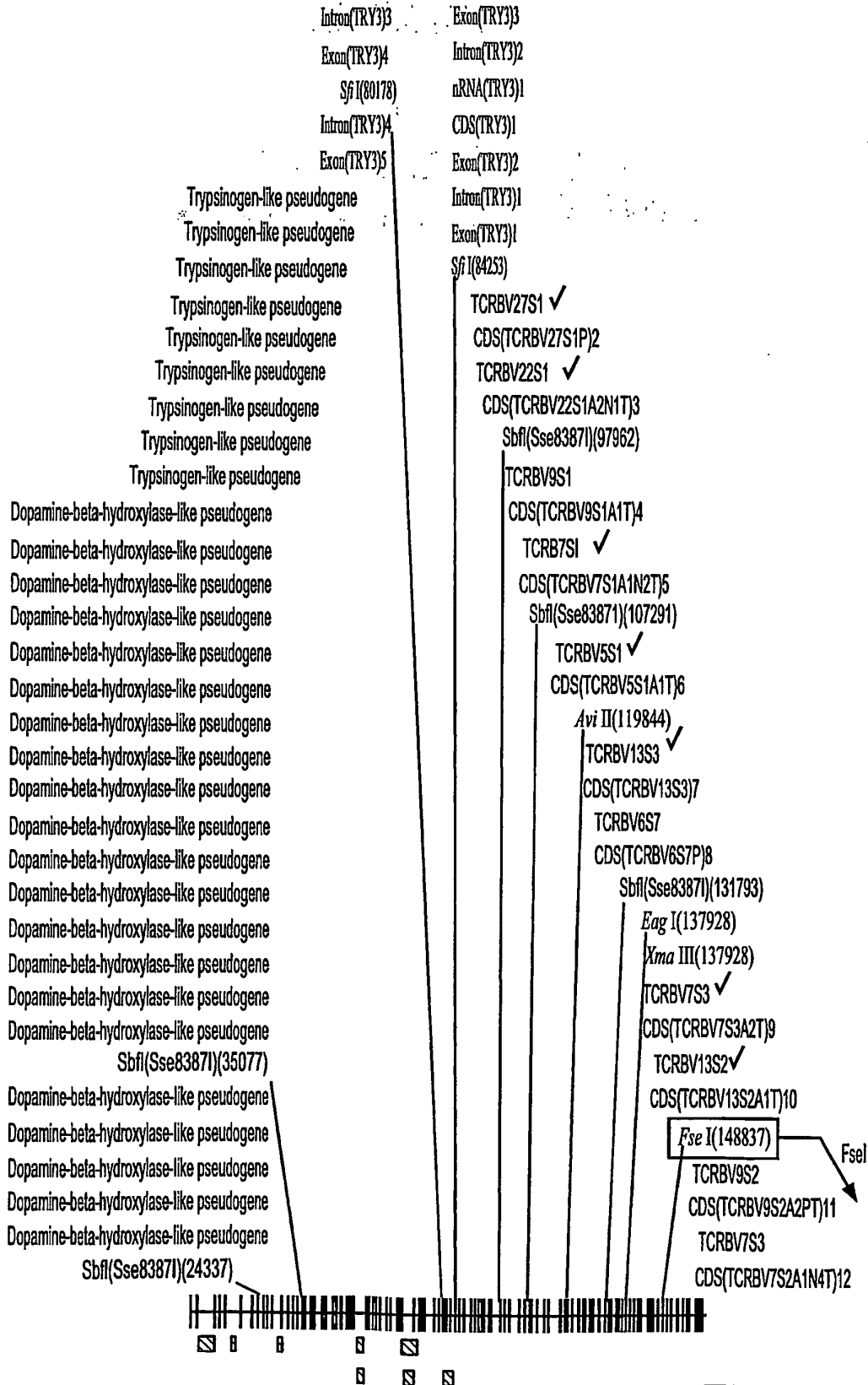
Fragment of U66059 161934 bp (molecule 267156 bp)
