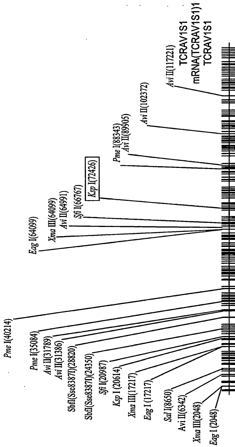
Fragment of HAUE000658 137784 bp (molecule 250529 bp)
