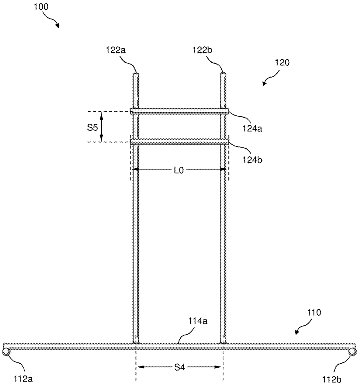
(FRONT VIEW)
